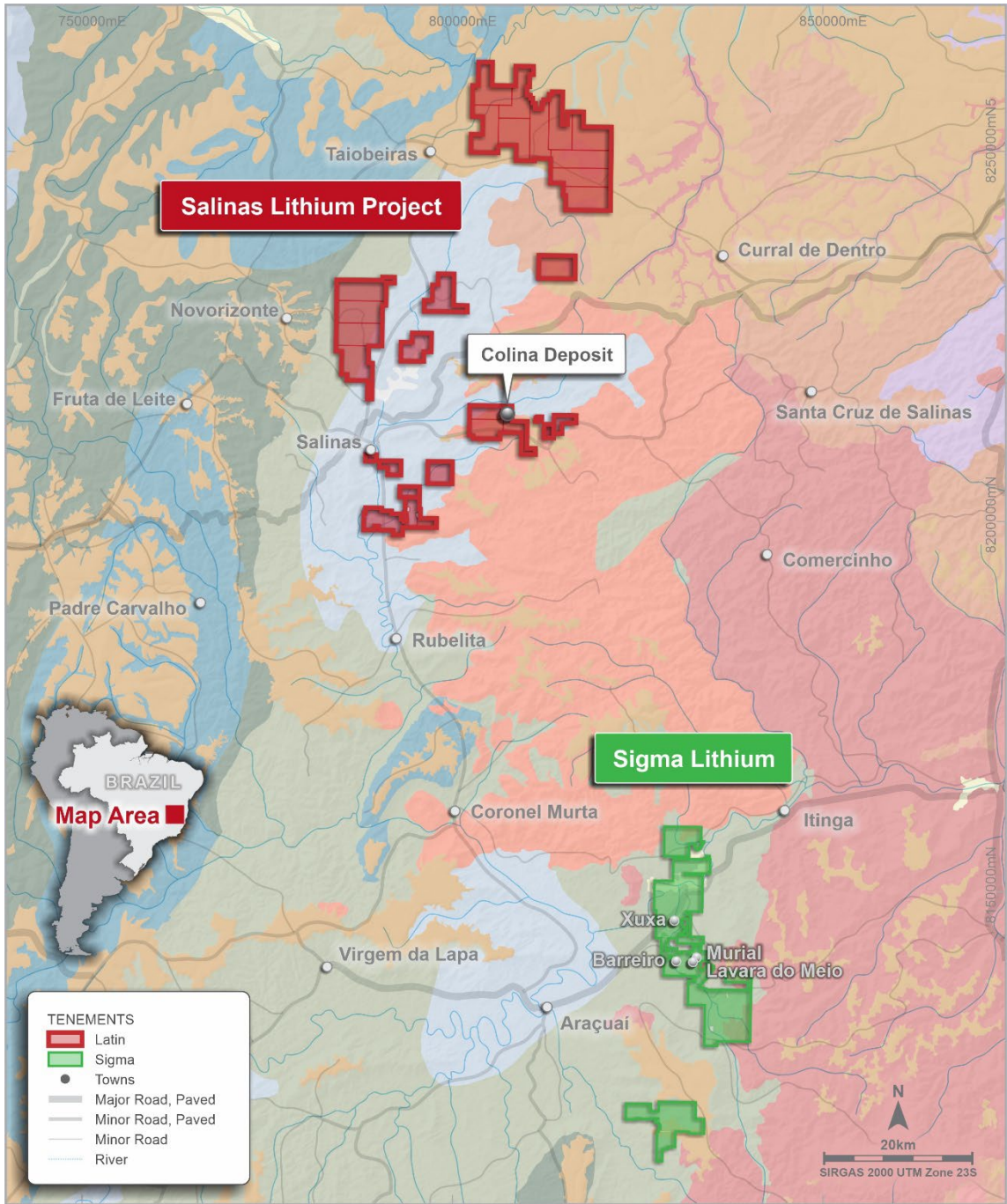
FIGURE 3 SALINAS LITHIUM PROJECT REGIONAL GEOLOGY AND TENURE
