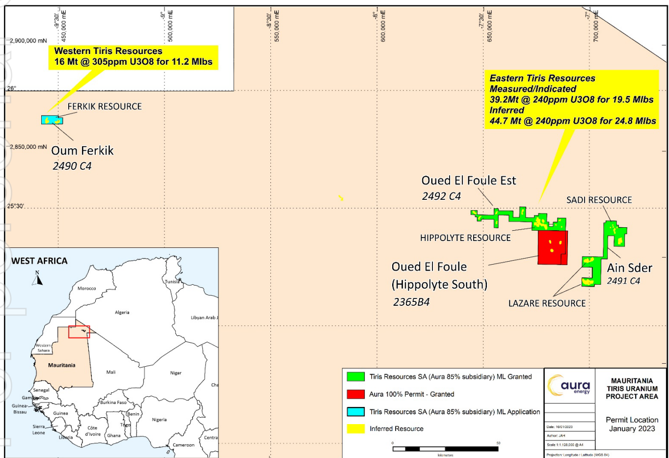
Figure 1 - Aura Energy Limited Distribution of Resources
