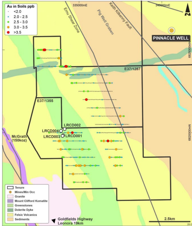
Figure 5 Area 2, Pinnacle Well Soil Geochemistry; Gold results
