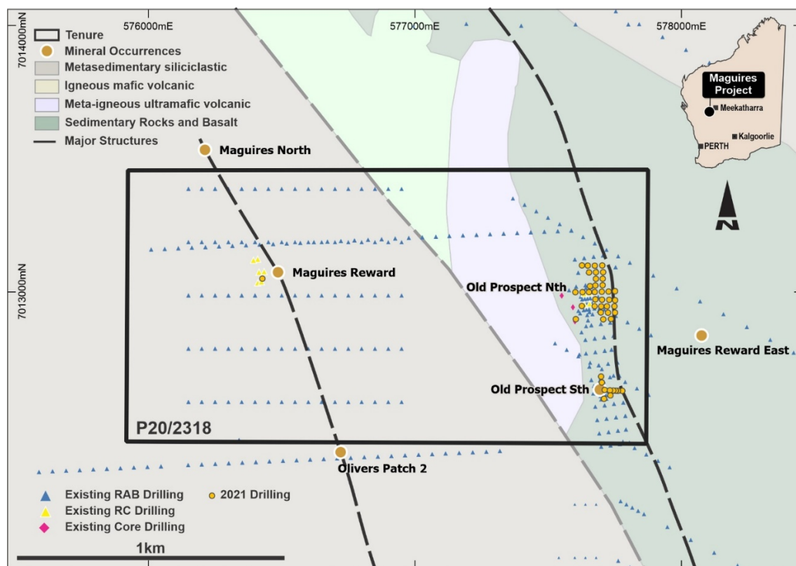
Figure 10 Maguires Reward – Tenure, Geology and Drilling Plan
