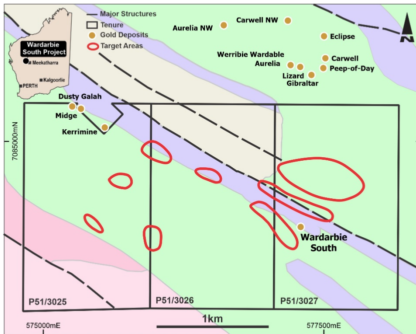
Figure 15 Wardarbie South - Tenure and Geology Plan
