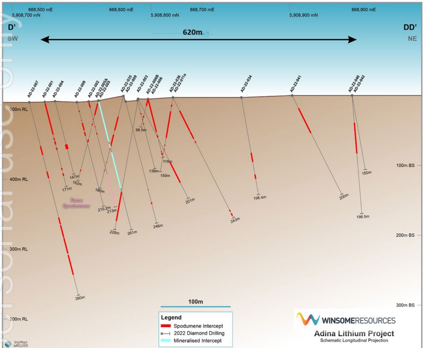
Figure 4: Long section view of Adina drilling program
