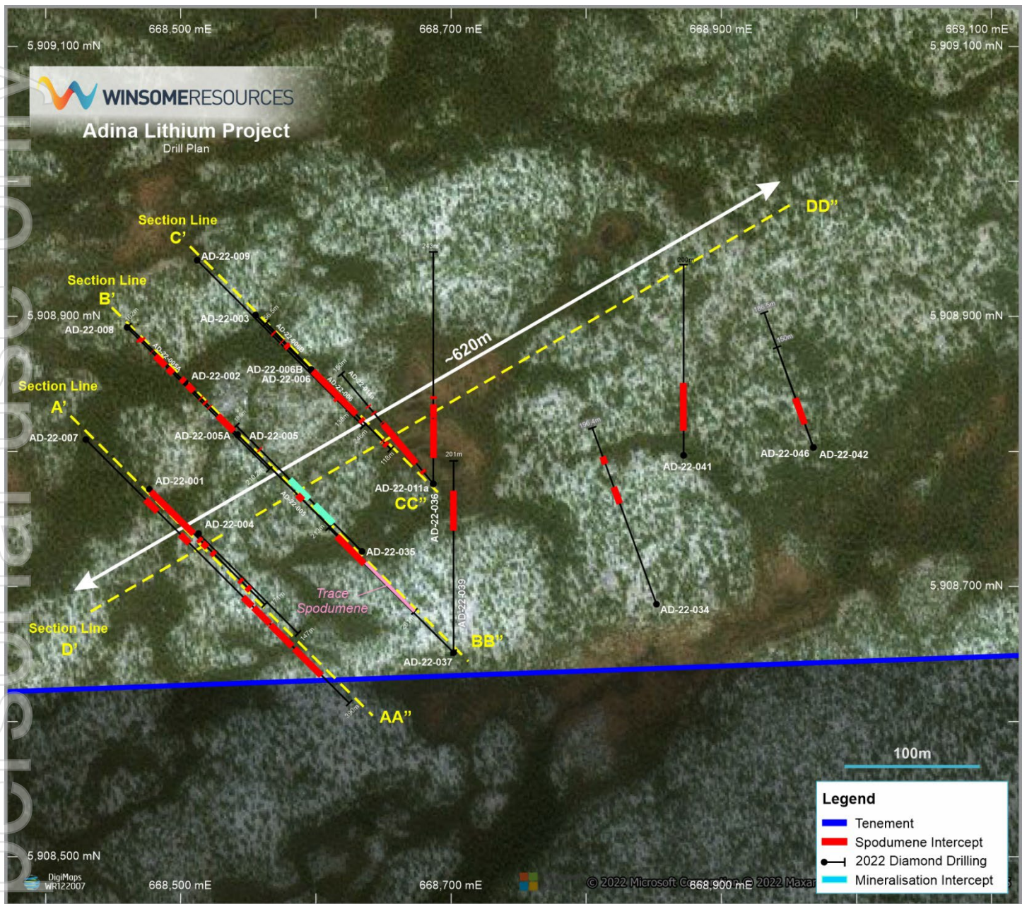
Figure 1: Plan view Adina diamond drilling campaign
