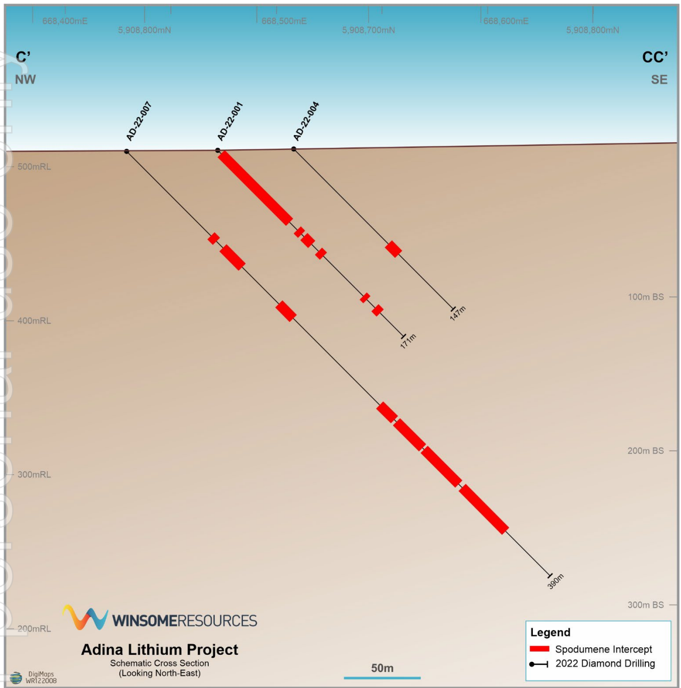
Figure 3: Section view looking North-East – Line C' – CC'
