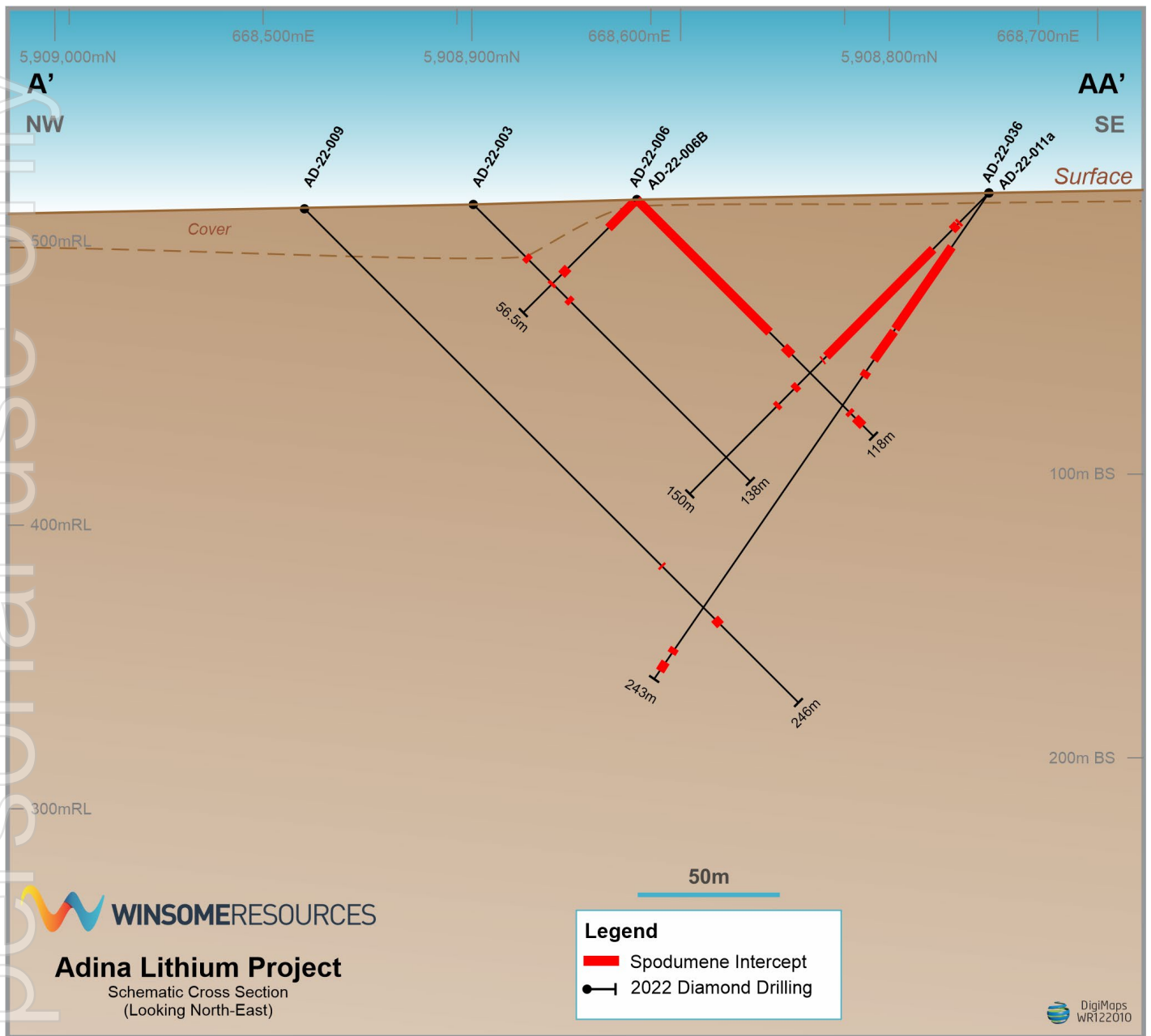
Figure 2: Section view looking North-East – Line A' – AA'
