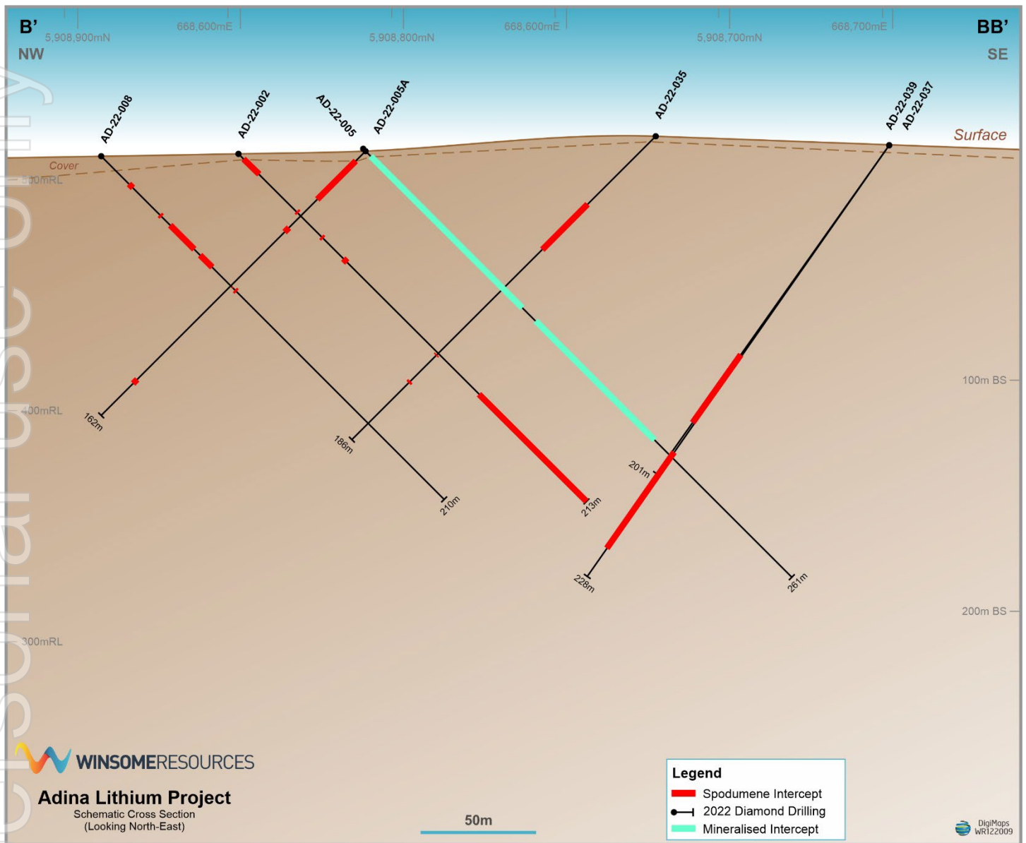
Figure 3: Section view looking North-East – Line B' – BB'
