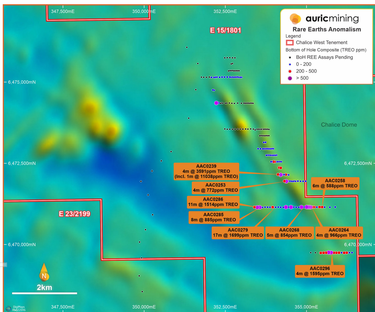
Figure 2: Total magnetics intensity (TMI) map from GSWA illustrating 7-km long magnetic anomalies at Chalice West which coincides with anomalous REE intervals.
