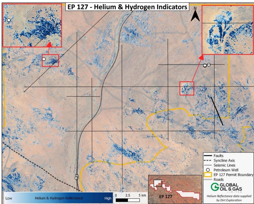
Figure 1 – Helium & Hydrogen Reflectance Data
