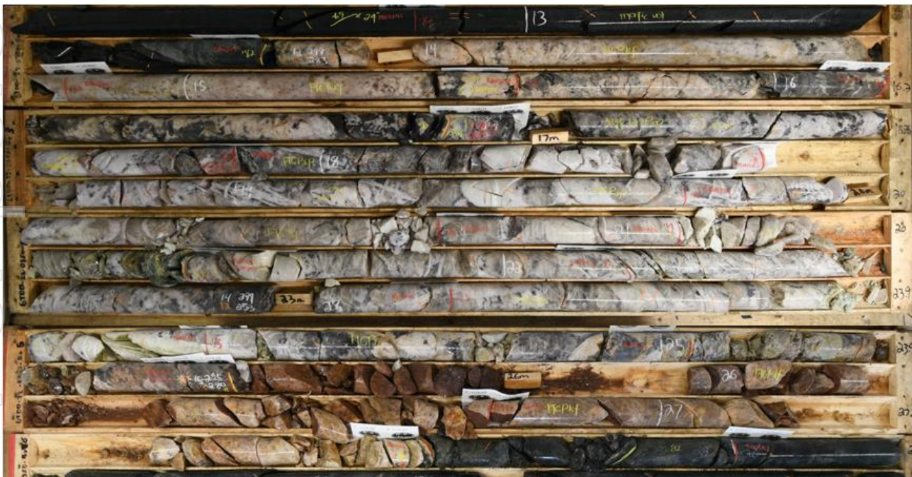
Figure 4: GTDD-22-0350 – example of coarse spodumene crystal laths within pegmatite mass (13.9m @ 1.53% Li 2 O)
