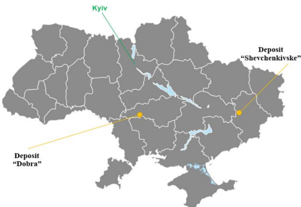
Figure 2 - Location of the deposit Shevchenkivske and Dobra in Ukraine
