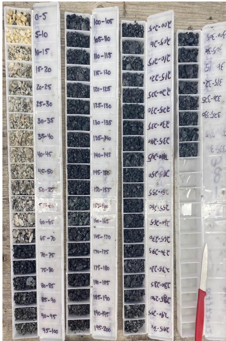
Figure 6 – Chip trays from RC drilling at Cancet showing the difference between pegmatite (white/gray) and surrounding amphibolite (black)
