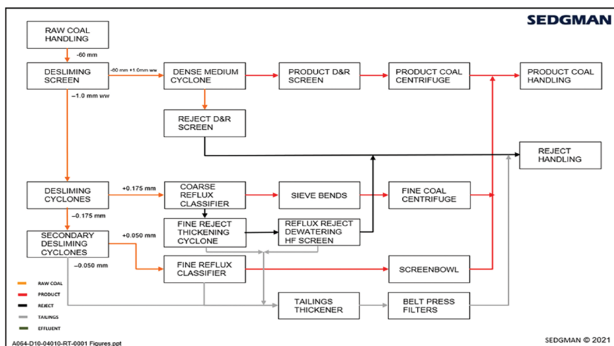
Figure 2: Ovoot CHPP Flowsheet.
