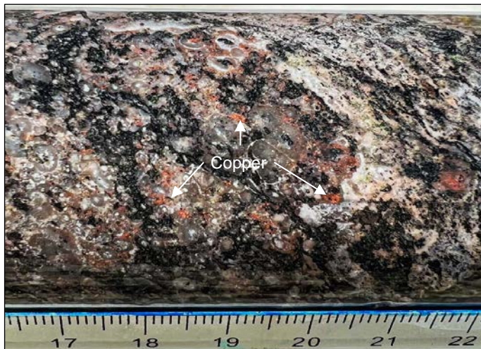
Figure 7b Breccia with disseminated native copper (orange) through the matrix. Strong biotite (black), silica (clear) and magnesite (white) alteration.
