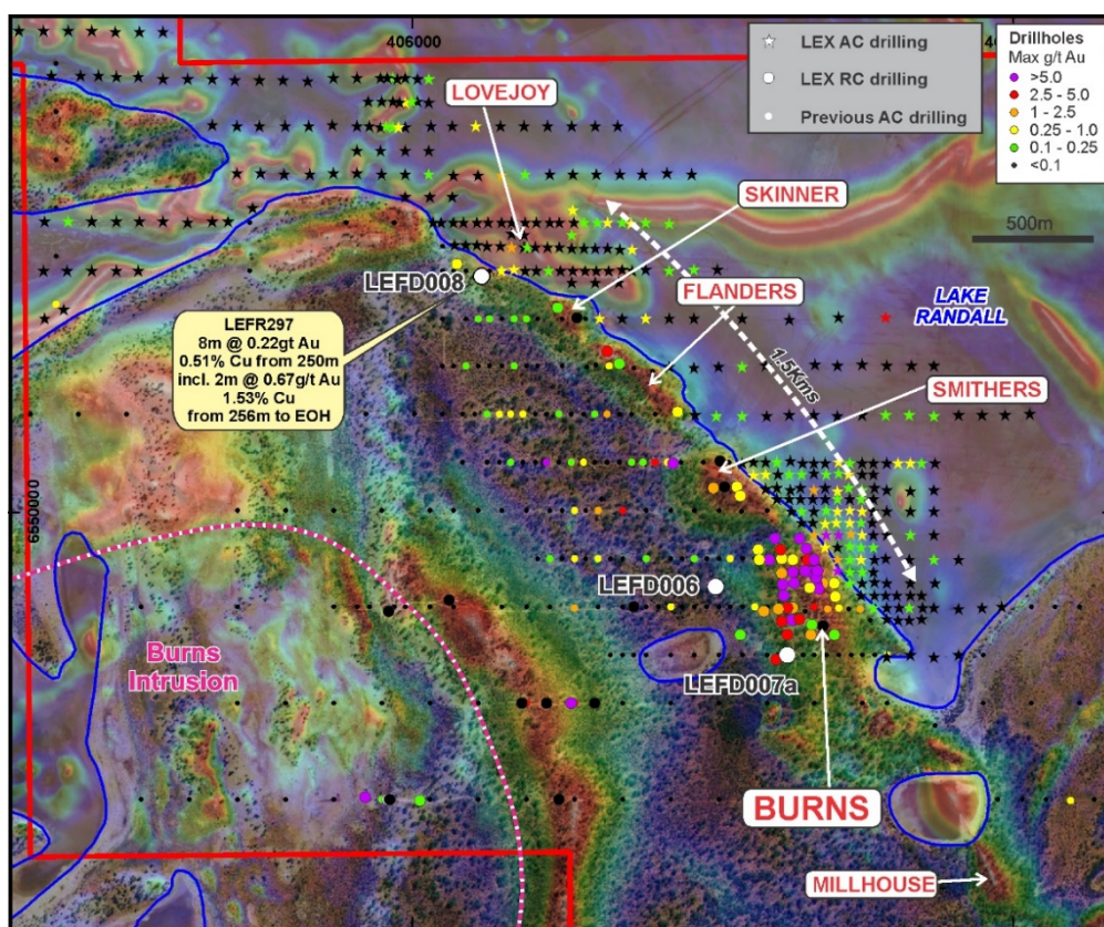
Figure 1 Combined satellite image with transparent TMI RTP aeromagnetic image highlighting the discrete magnetic anomalies along strike of Burns (warm colours represent rocks beneath the surface with higher magnetite content). Coloured and black dots represent historical AC drill holes. The recent diamond drill holes are highlighted. Refer to Figure 2 for the Lovejoy drill section.
