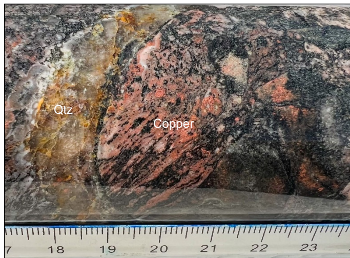
Figure 7d Breccia with native copper (orange), quartz vein to the left with crystalline native copper inside, strong biotite (black) and silica alteration.
