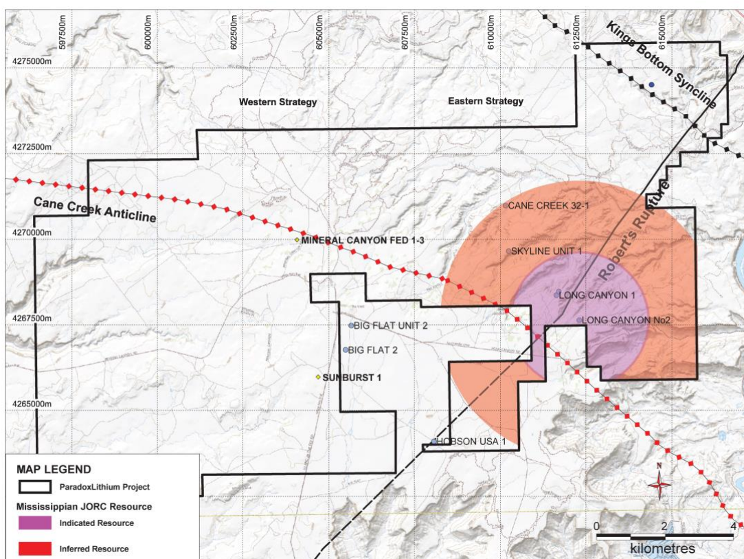
Figure 1: Plan showing the Resource AOI, and the Roberts Rupture Cane Creek Anticline.
