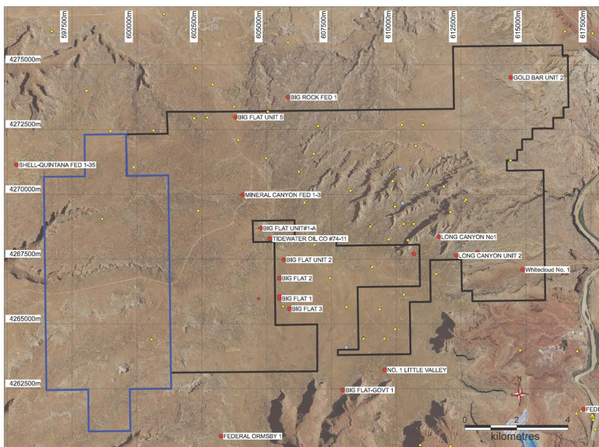
Figure 2: Plan showing the well locations that drilled into the Mississippian Units at the Paradox Lithium Project.
