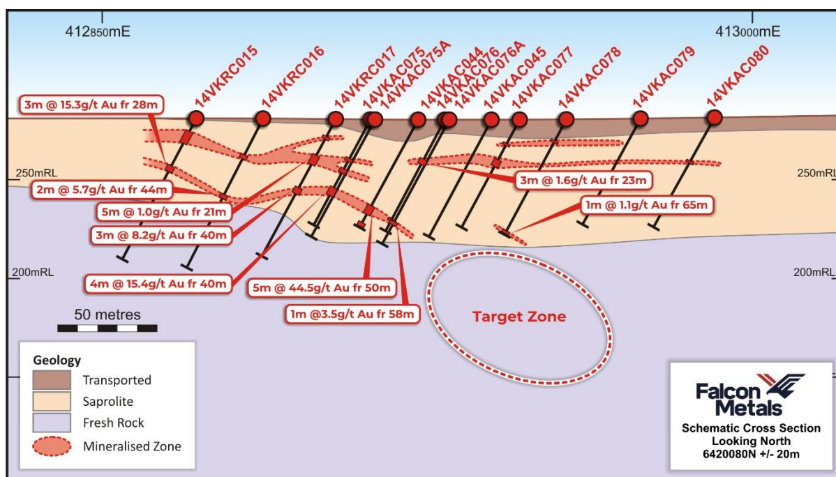
Figure 3 Beaker 2 Cross Section
