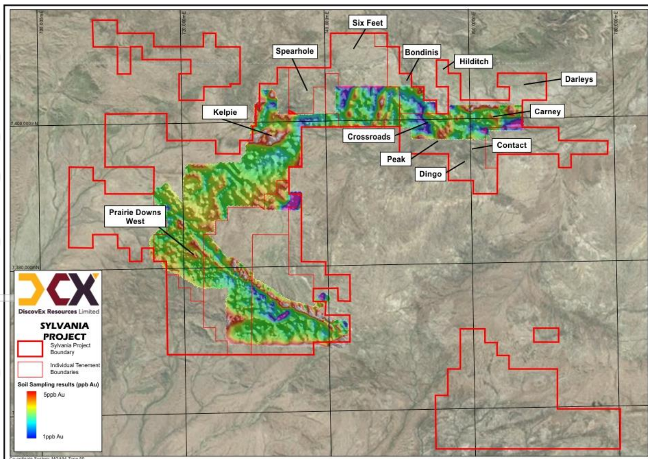
Figure 3: The Sylvania Project showing an amalgamated (historic data plus latest data) gravity image.
