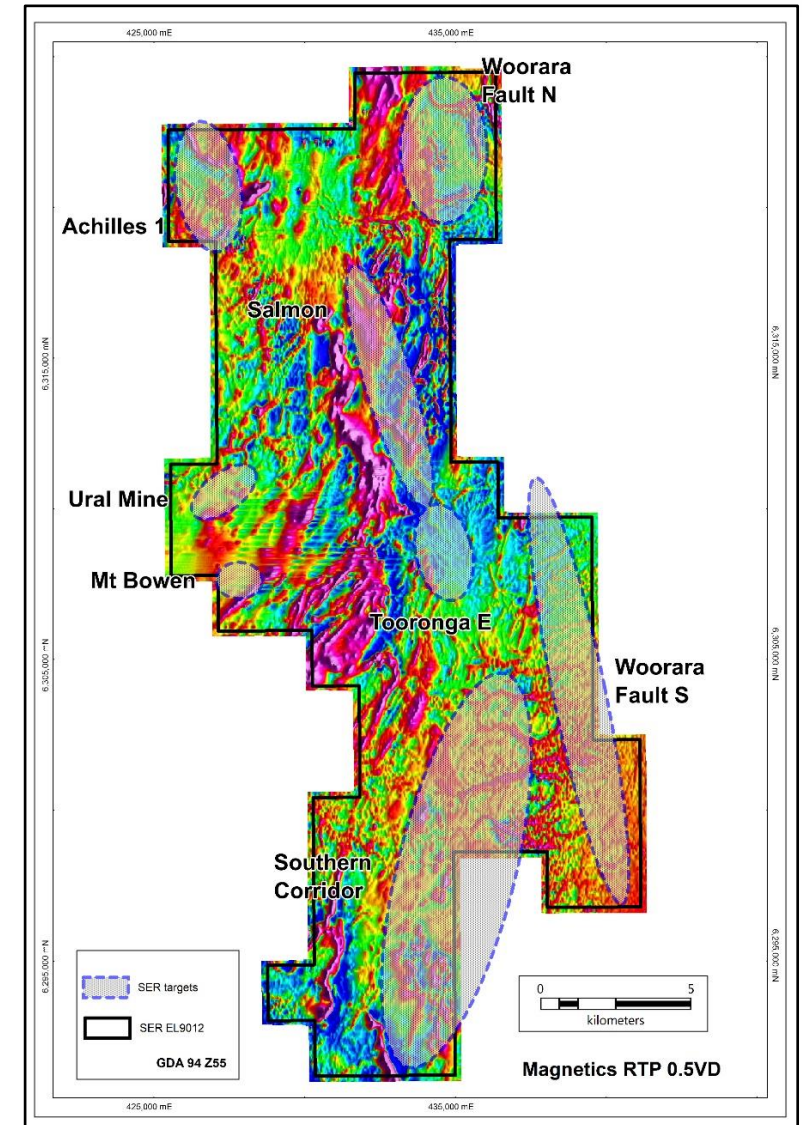
South Cobar targets over 0.5VD RTP Magnetics
