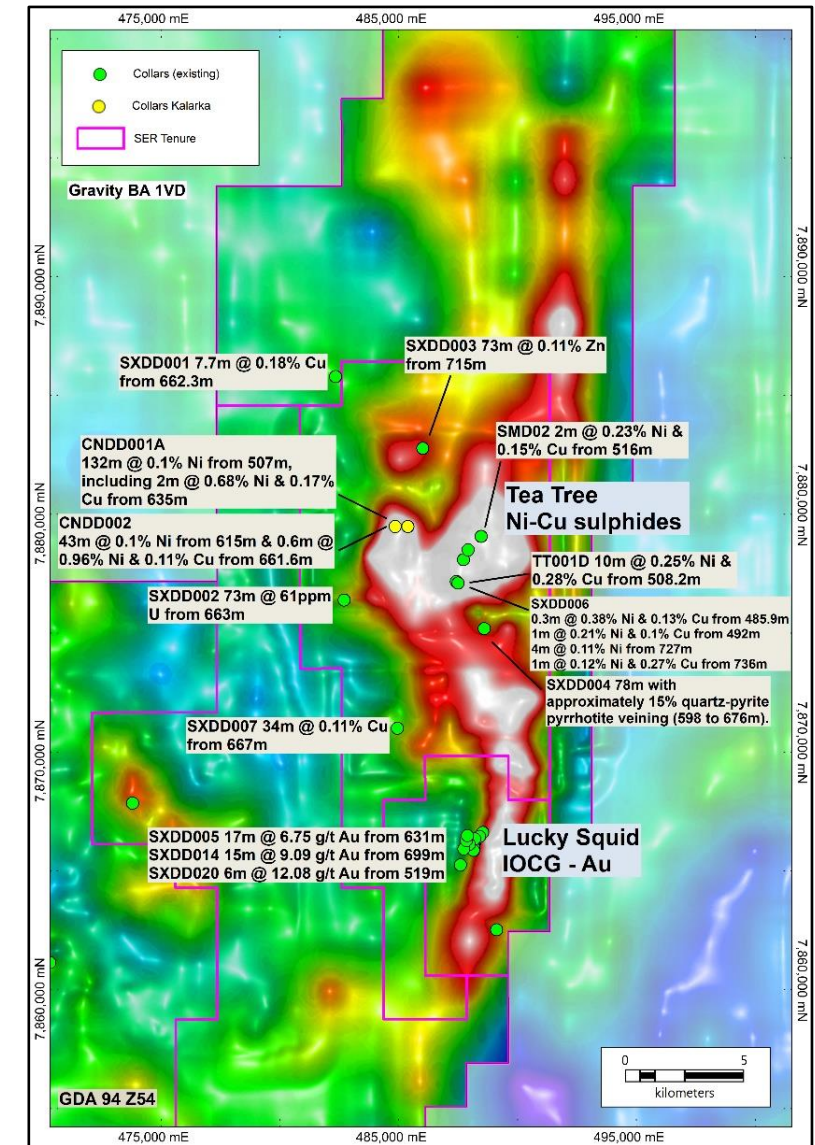
Bouguer Gravity 1 VD image with historical intercepts
