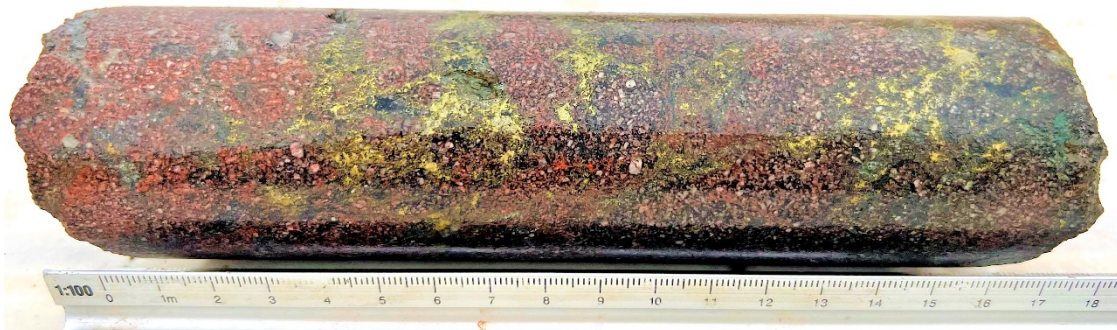
Figure 5 LEFD006 interval 435.6-435.8m showing Burns diorite porphyry altered by pervasive hematite, cross-cut by chalcopyrite and pyrite stringer veining (LEX ASX release 1 August 2022).
