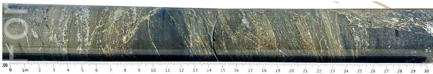
Figure 6 LEFD006 interval 1031.95-1032.25 4 Carbonate and quartz altered siltstone. Sub massive pyrite and pyrrhotite with rare chalcopyrite
