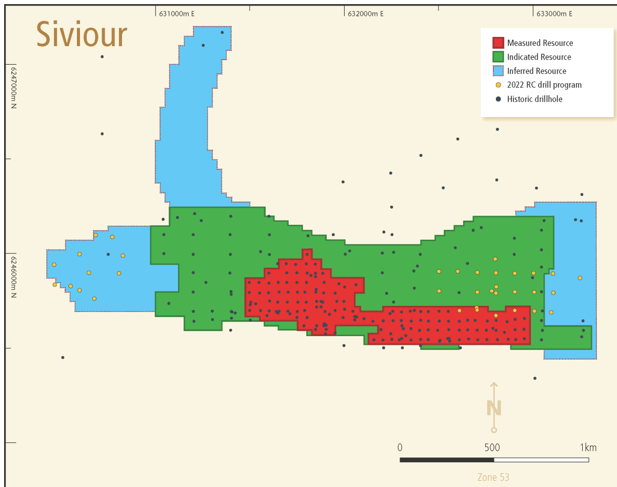
Figure 1. 2022 drill holes (yellow) and historic drill holes (black) within the Mineral Resource classification areas
