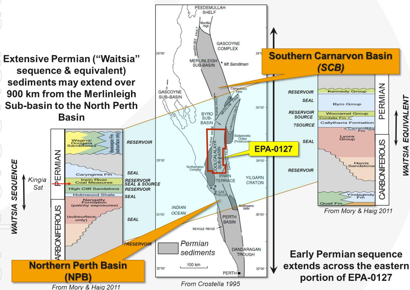
Figure 3. STP-EPA-0127 map highlighting Permian sequence
