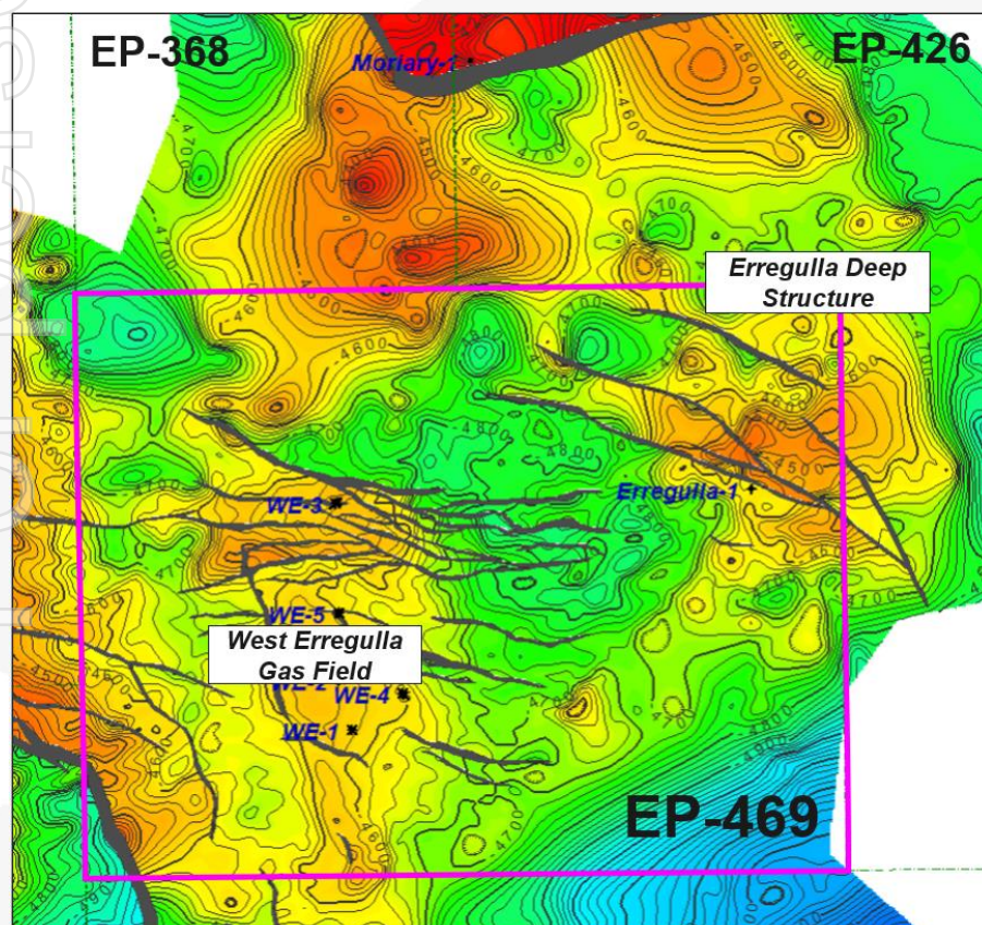
Figure 2. Top Kingia depth map
