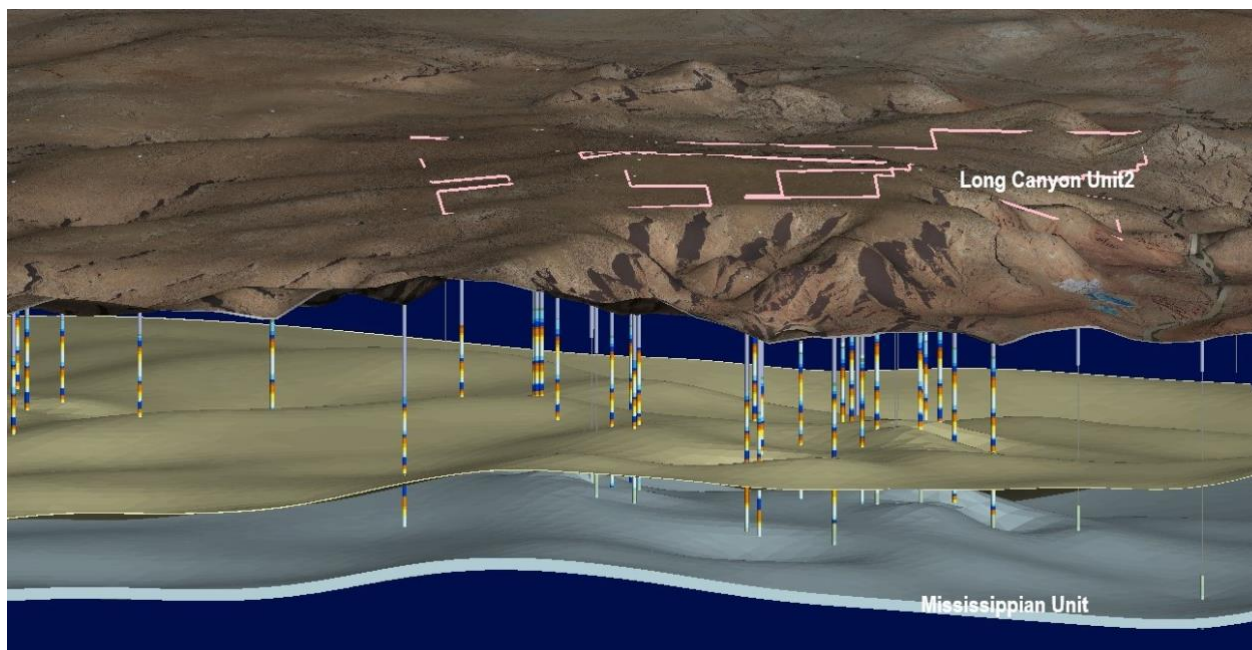
Figure 4: 3D model showing the thicknesses of the Clastic Zone 31 and Leadville Limestone units.
