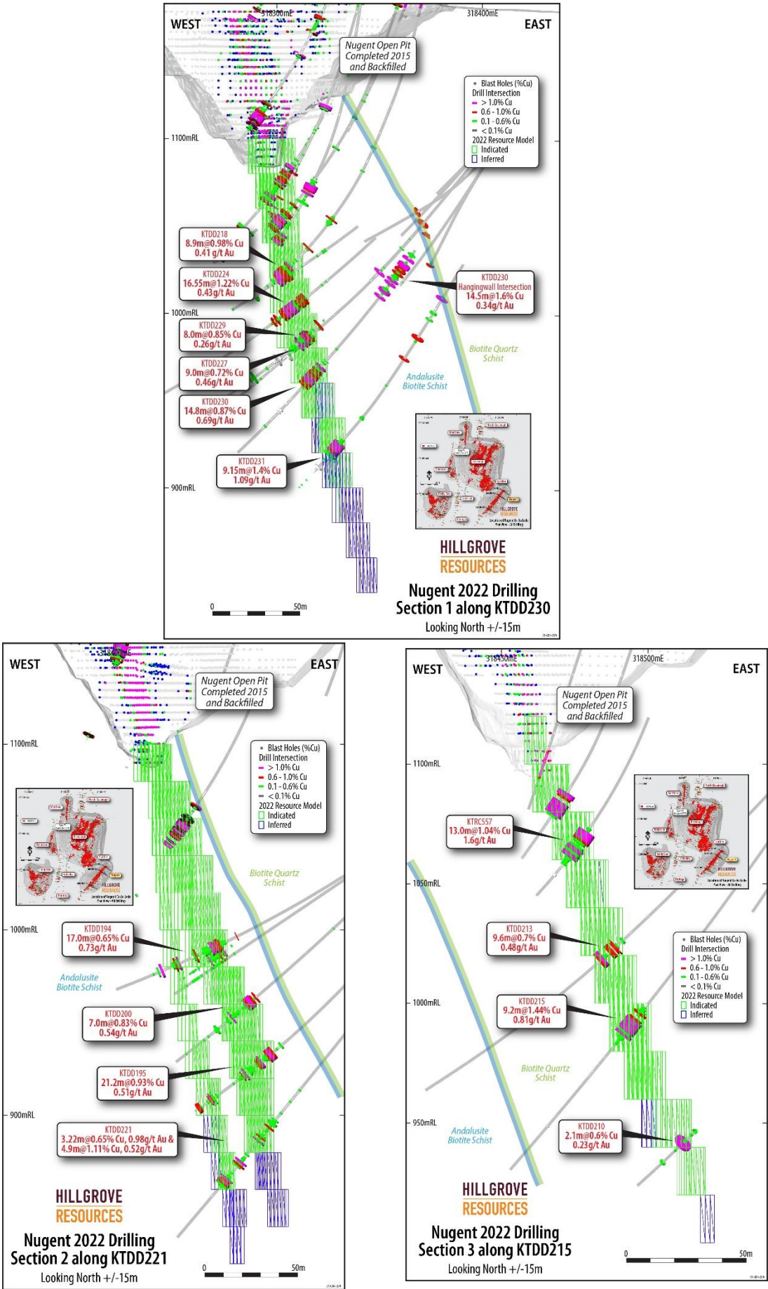
Figure 3 Cross sections of 2022 MRE showing classification
