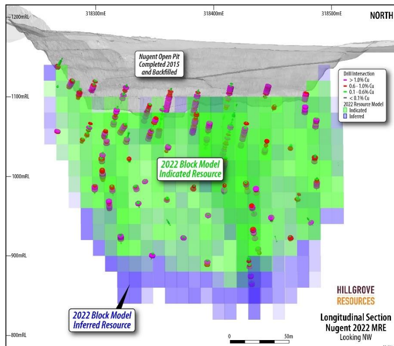
Figure 2 Long section through the 2022 MRE showing the classification
