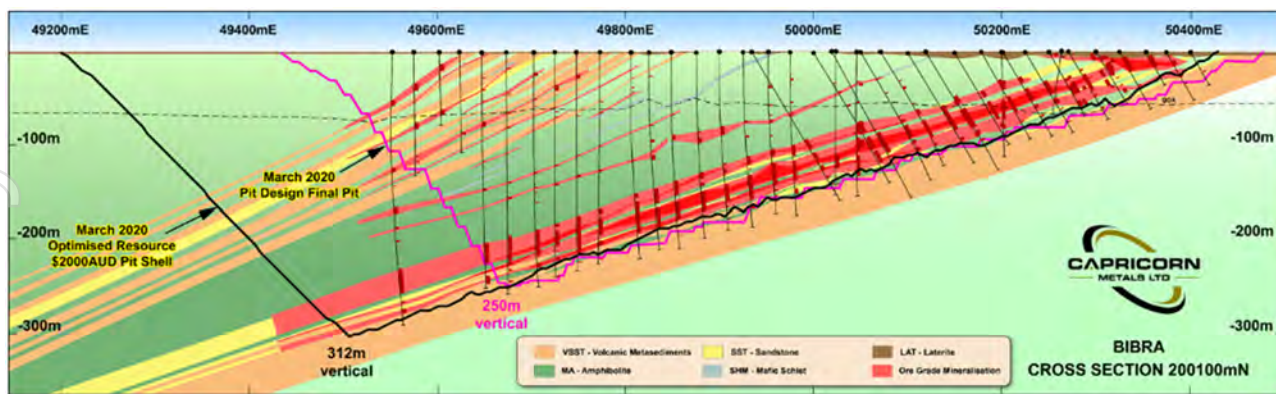
Figure 16. Bibra Open Pit section
