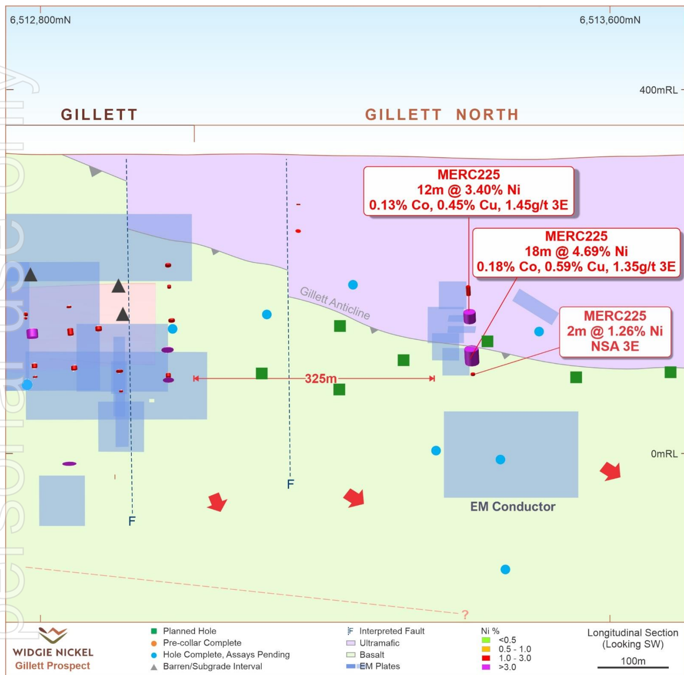
Figure 1 – Long section looking south-west showing recent drilling at Gillett North, MERC225 and DHEM conductors
