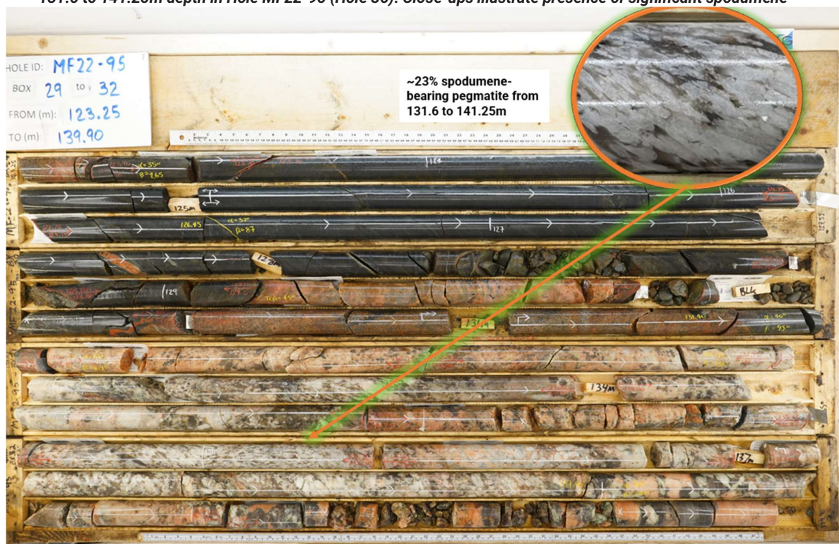
Figure 3: White pegmatite hosts approximately 23% of fine to large, white-grey, spodumene laths intersected from 131.6 to 141.25m depth in Hole MF22-95 (Hole 36). Close-ups illustrate presence of significant spodumene
