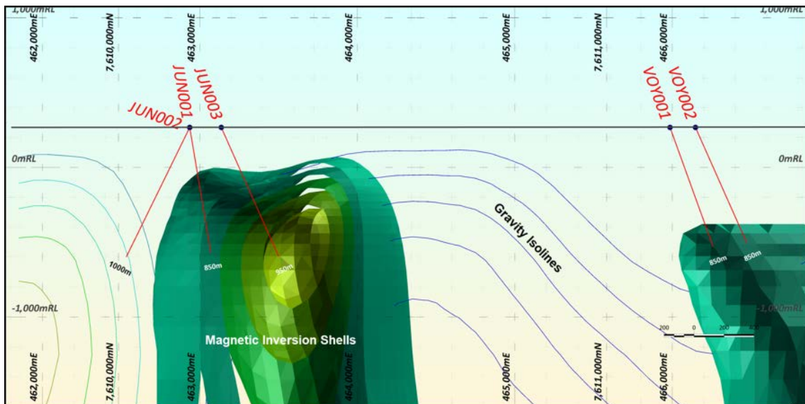
Figure 7: Oblique section A- A' view of Juno and Voyager magnetic signatures. A distinctive gravity trough forms in the Juno area, with a strong off-shoulder gravity anomaly forming to the southwest. Refer to Figure 4 for location of section.
