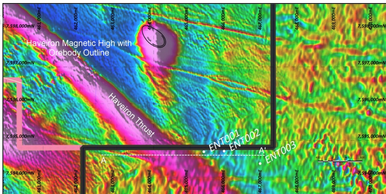
Figure 8: Location of the three holes planned to be drilled at Enterprise. These holes are targeting the Haviron Thrust south of the Haviron Deposit. Refer to Figure 9 for section A – A' details.
