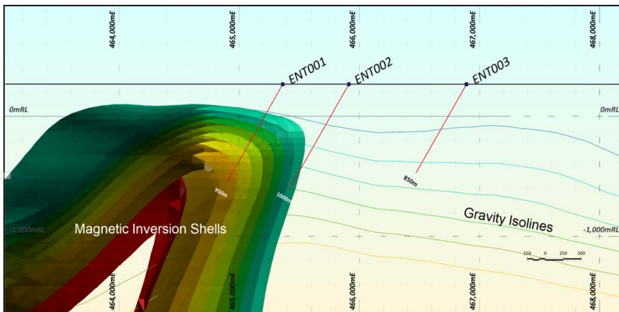
Figure 9: Section A – A' looking north showing the magnetic shells defining the Haviron Thrust and proposed holes. Gravity lines in this area are relatively flat lying with a raised ridge coincident with the strong mag signature at the thrust. Refer to Figure 6 for section location.
