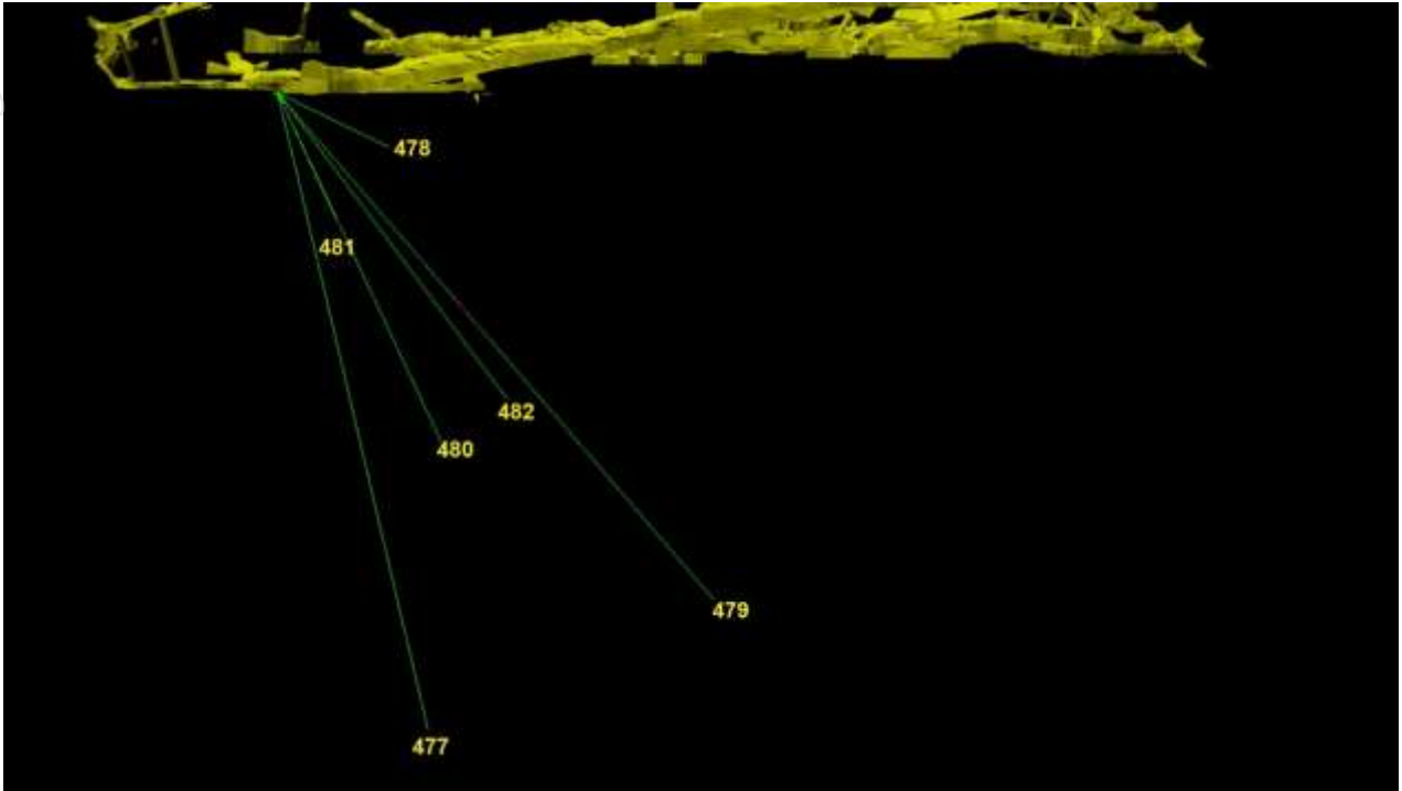
General long section highlighting recent drillholes beneath current development drive, looking West
