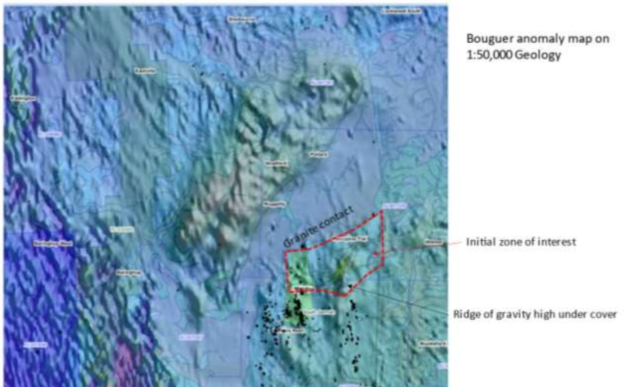
Figure 3: Gravity anomaly map showing prospective gravity ridges obscured by shallow cover soils located to the east of Maldon but within the Kaiser exploration licence application (EL7029).
