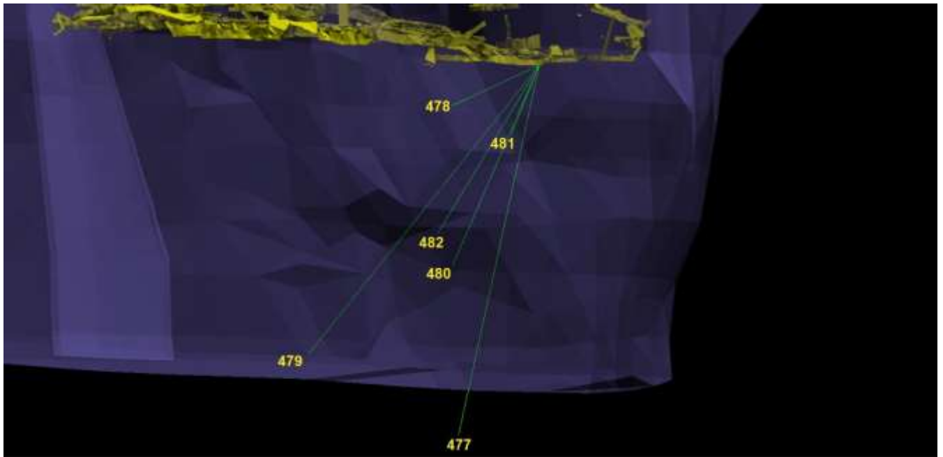
Figure 2: Long section looking west showing drilling traces (green), workings and the interpreted main dyke shape (purple)
