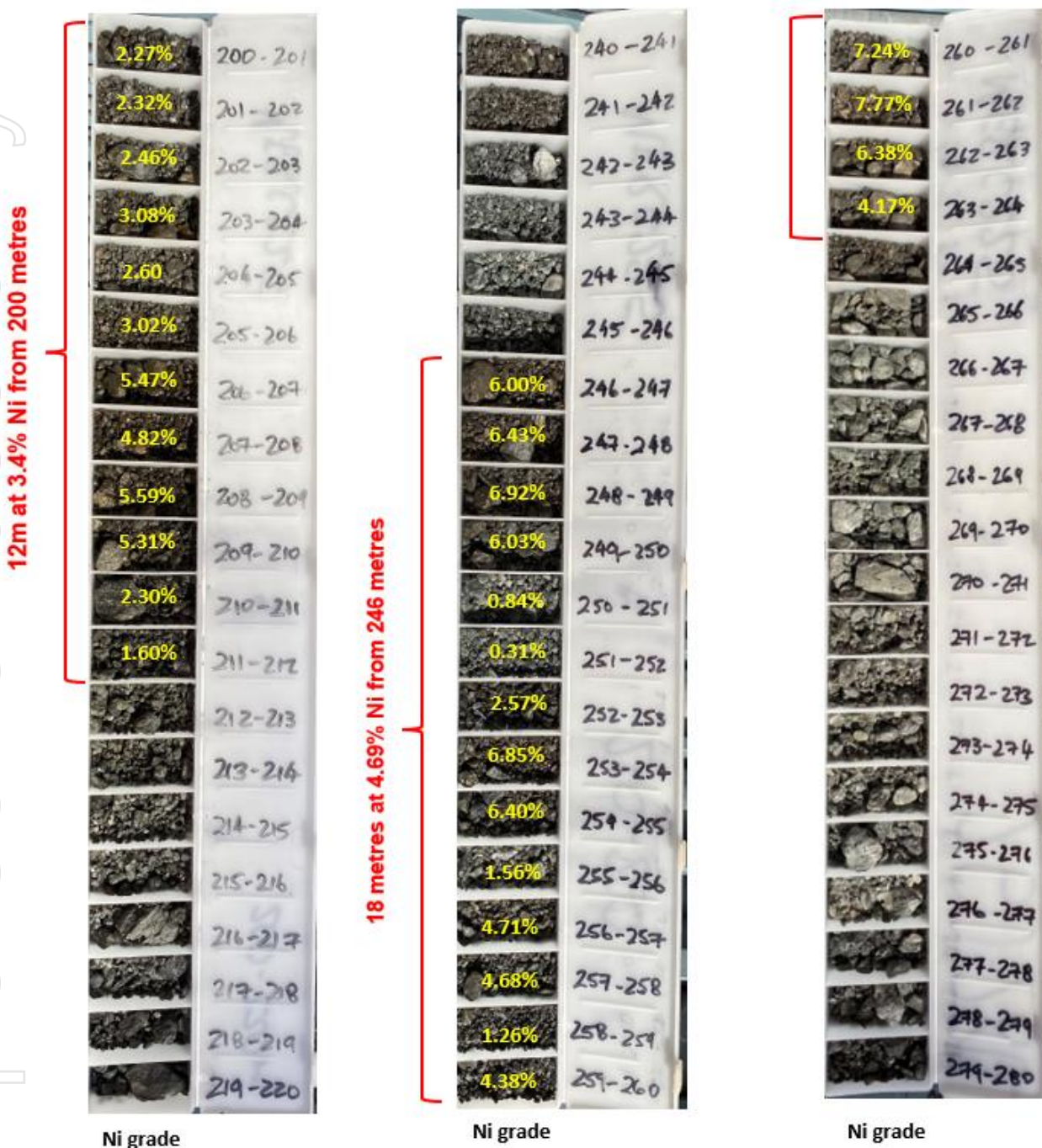
Figure 1 – MERC225 RC chips showing massive sulphide intervals and assays
