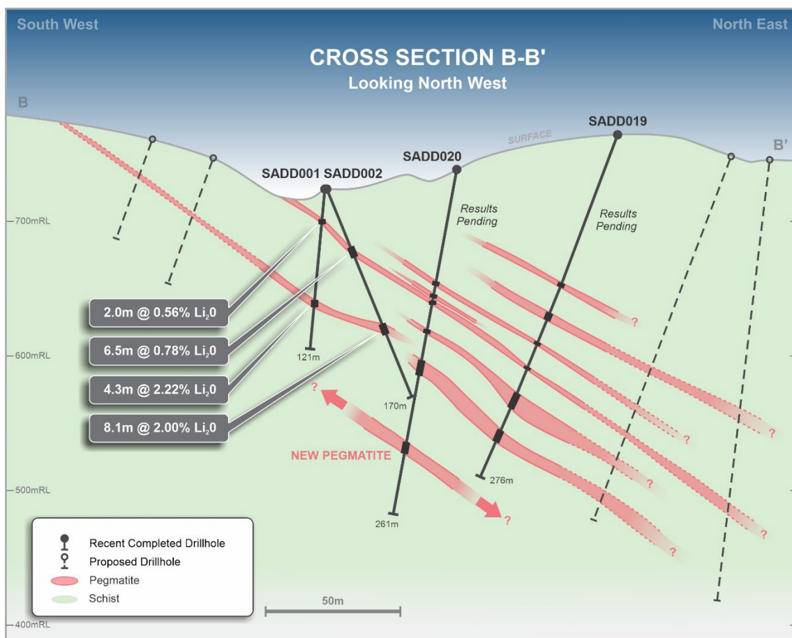
Figure 4: Drill section B-B' showing completed and planned drill holes, and logged pegmatites for holes SADD019 and SADD020 (results pending) 6
