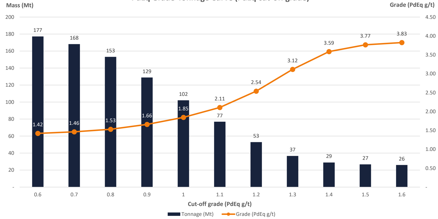
Figure Two | Pantom PdEq Grade-Tonnage Curve
