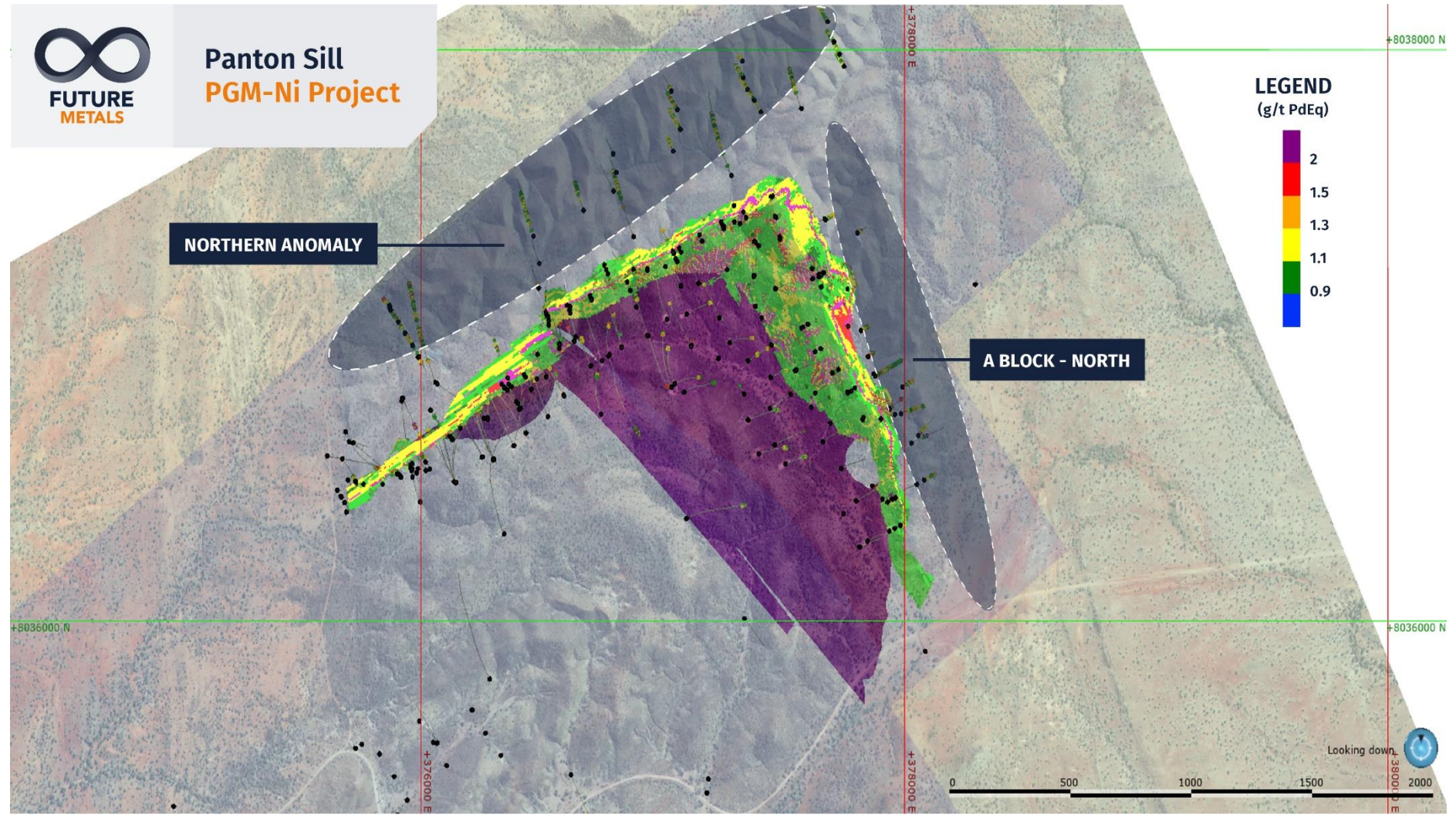
Figure Nine | Plan View of Panton including target zones for near-surface exploration
