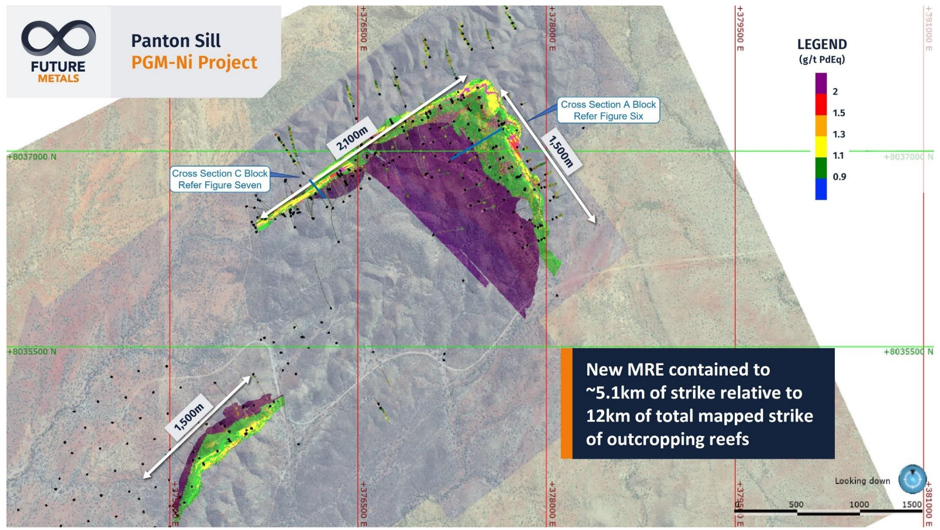
Figure Five | Plan View of Panton including MRE area
