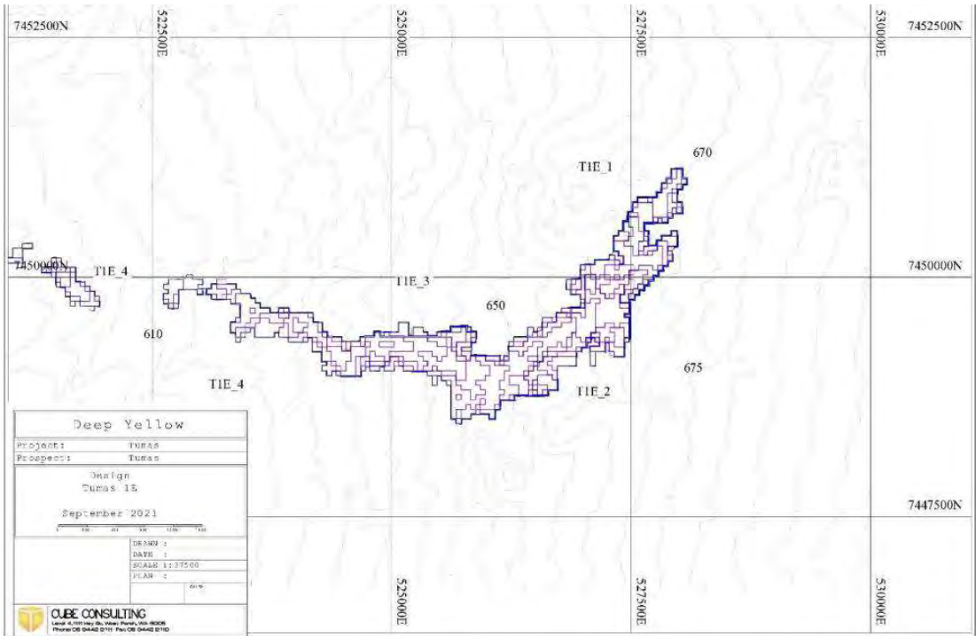
Figure 3-10: Tumas 1E pit design
