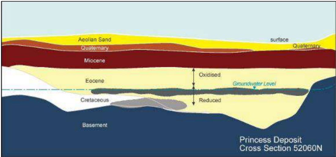
Figure 2-5: Simplified cross section of the Princess deposit
