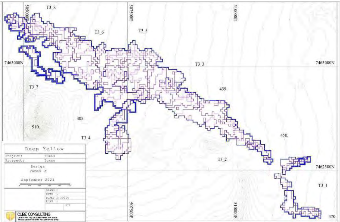
Figure 3-9: Tumas 3 pit design
