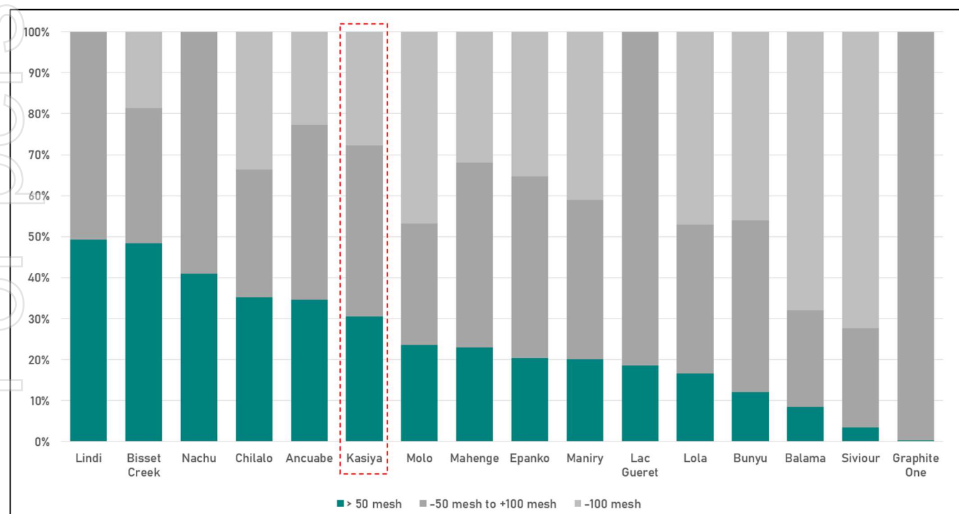
Figure 4: Flake Distribution of various graphite projects (Sources: Company reports)
