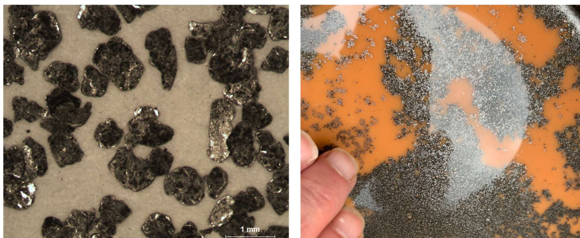
Figures 6 & 7: Very coarse-flake graphite in +600µm sample fraction (L), graphite floating on soaking drill sample (R)
