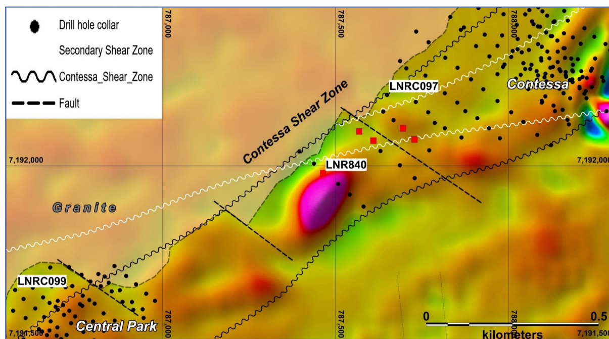
Figure 1 Contessa shear zone showing “bulls eye” magnetic anomaly and adjacent transition zone gold anomalies in aircore drilling (red dots). Magnetic image RTP2VD, MGA94 zone 50.
