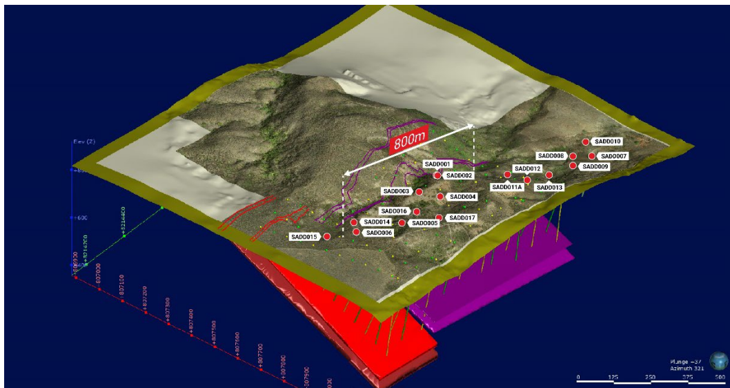
Figure 2: Oblique projection of the Colina Prospect area showing existing drill collars (red) and the planned (green/ yellow) drill collars of the resource definition drilling campaign
