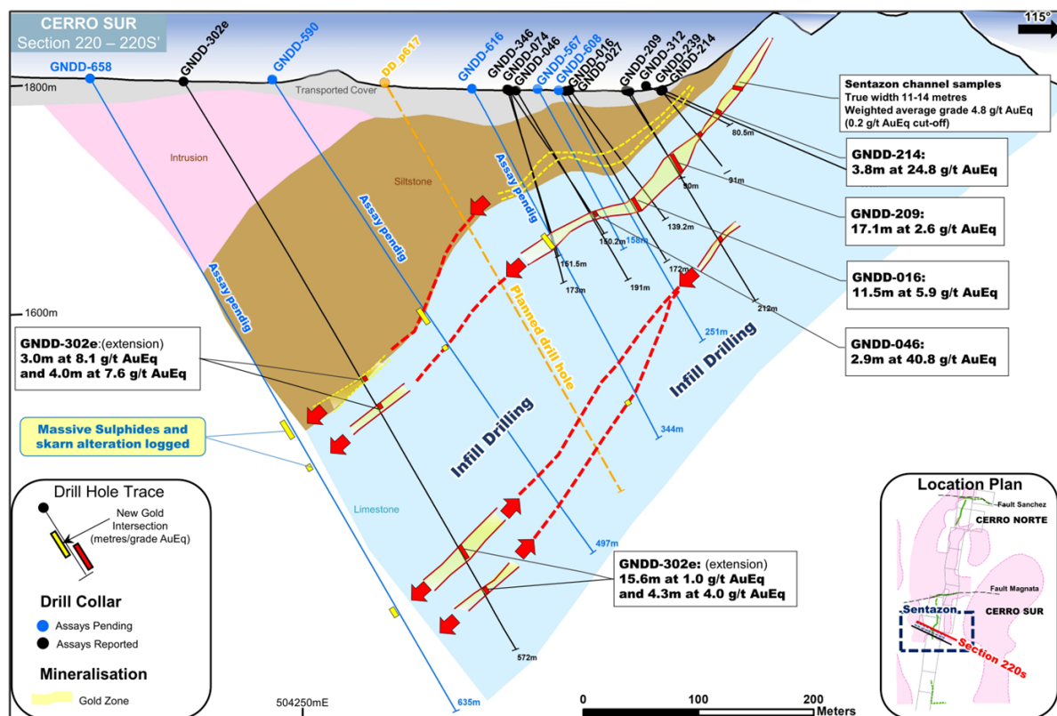
Section 1 - Showing Interpreted Geology
