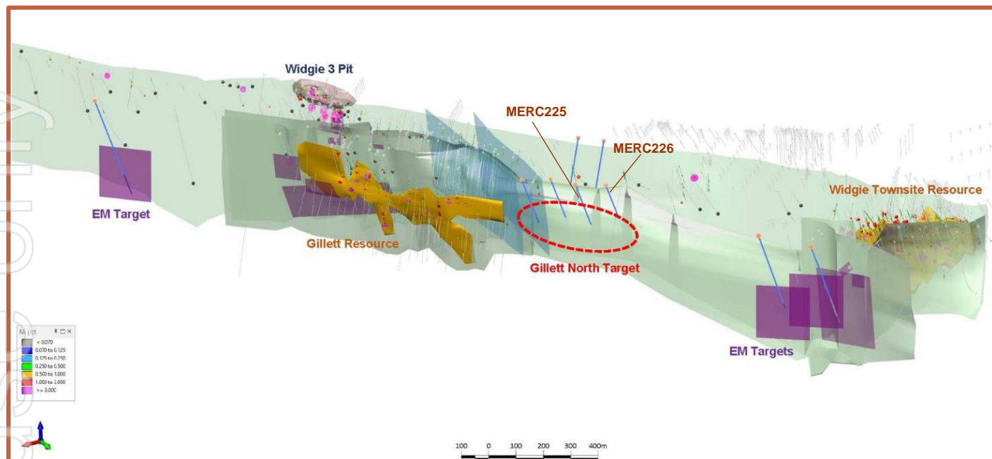
Figure 1– Oblique long section looking south-west showing Gillett North target proximal to the Gillett & Widgie Townsite Mineralisation
