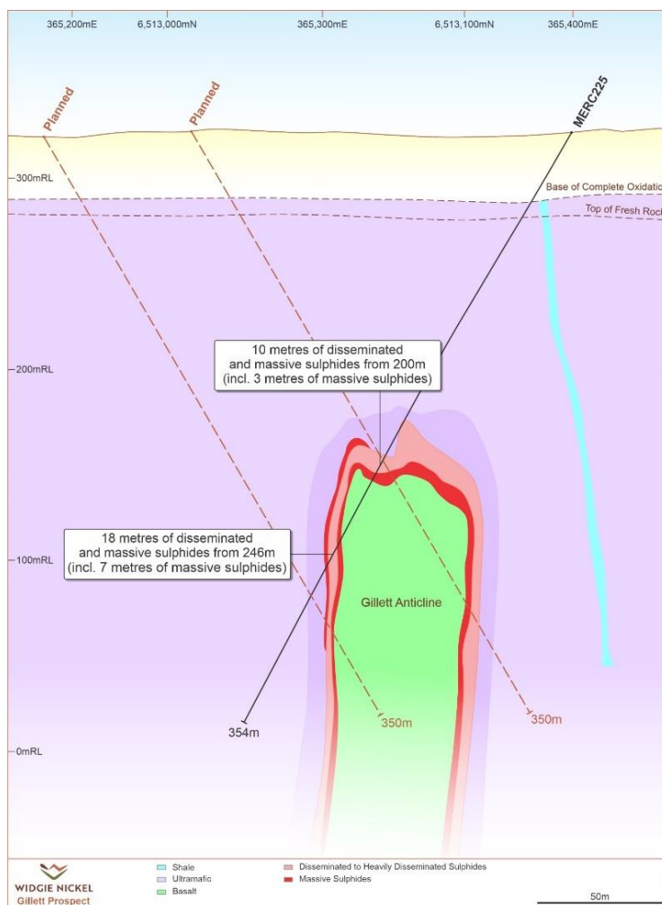
Figure 3 - Gillett North cross-section (looking NW), showing RC hole MERC225 and geological interpretation
