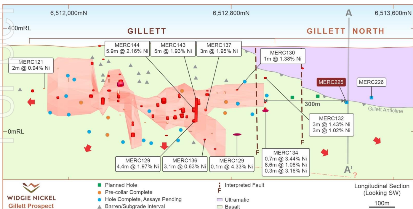
Figure 4 – Gillett long-section (looking SW), showing Gillett North sulphide intervals
