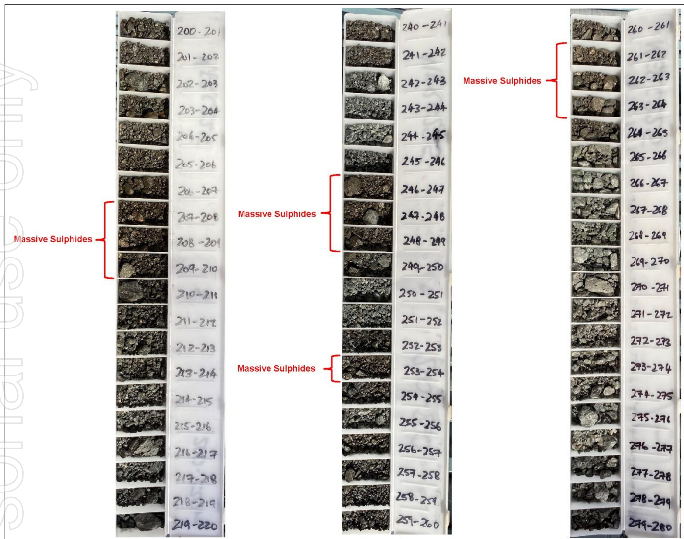
Figure 2 – Gillett North – MERC225 RC chips showing massive sulphide intervals
