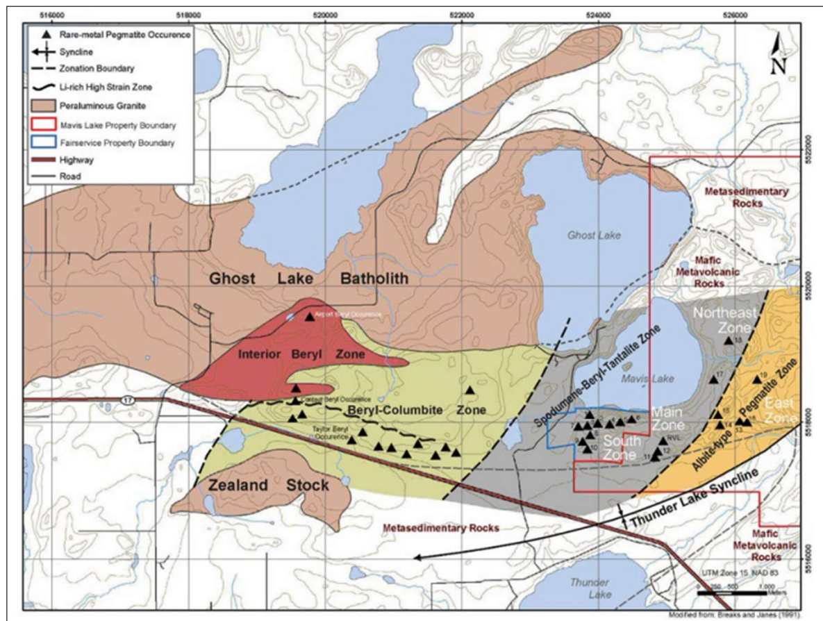
Figure 12: Regional zonation of Mavis Lake Pegmatite group
