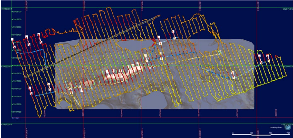
Figure 5 – Planned drill holes in white overlaid by Magnetic Survey results
