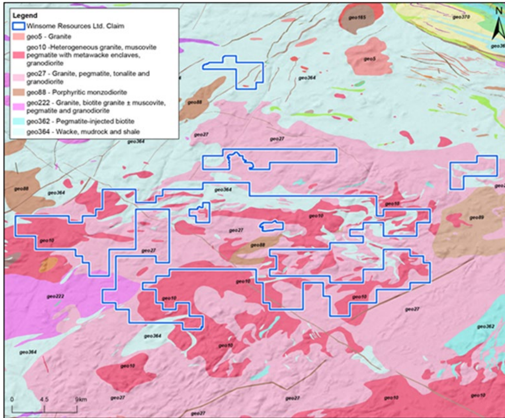
Figure 2 – Decelles regional geology
