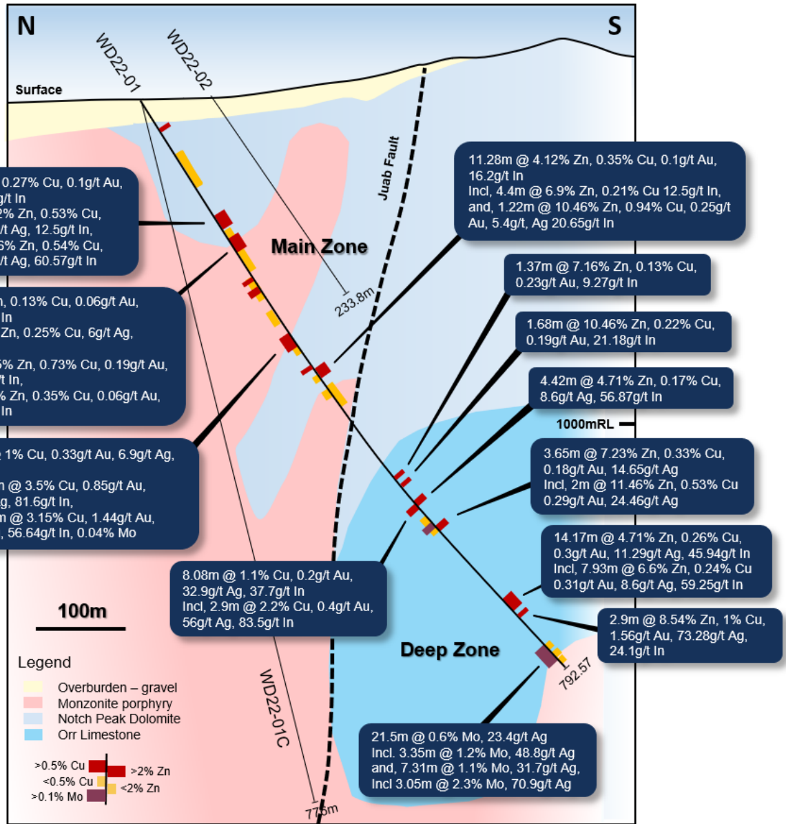
Figure 1: Schematic geological section at 288850E showing main geological units and drilling. Only significant intervals of Cu, Zn and Mo are shown (Table 1) with lower grade mineralisation highlighted in orange.
