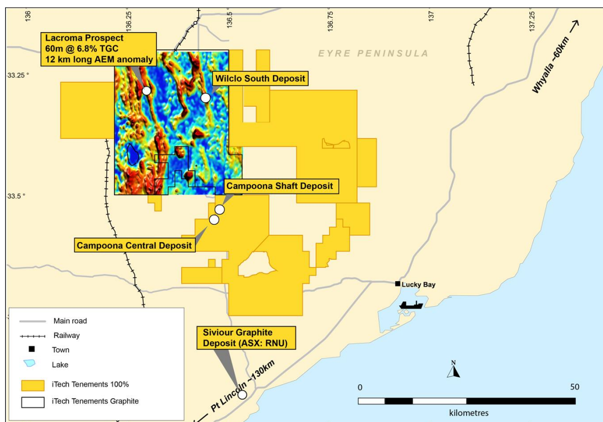
Figure 3. Location of graphite deposits and prospects with airborne electromagnetic image on EL6643 – Eyre Peninsula, South Australia
