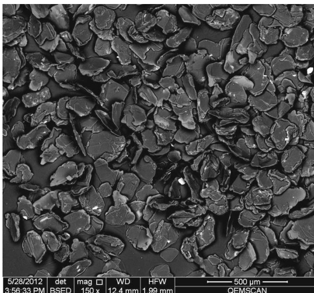
Figure 1. QEMSCAN image of flake graphite
