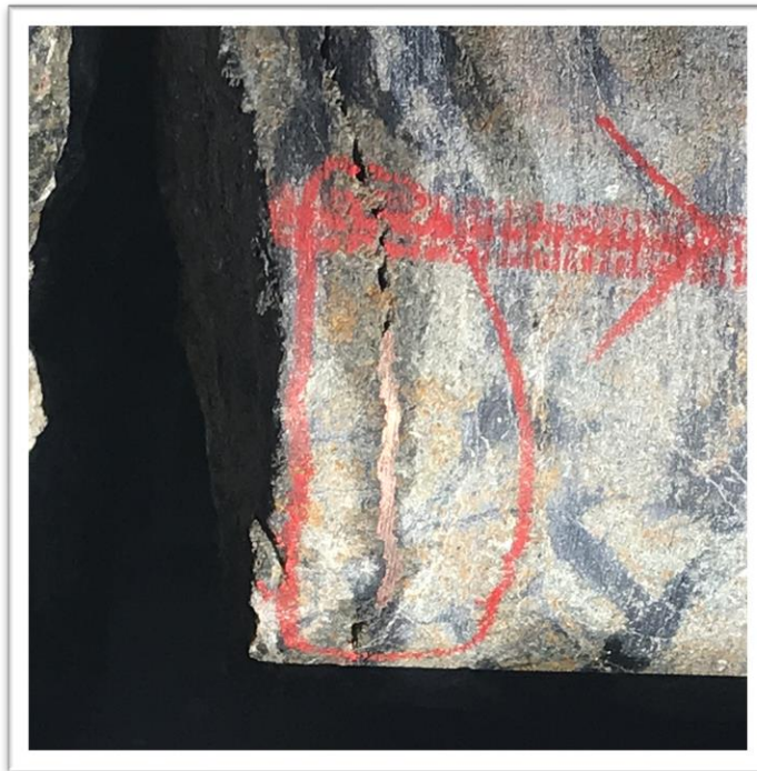
Figure 1 – Diamond Hole -NRDD002 - Native copper – 51.67m
