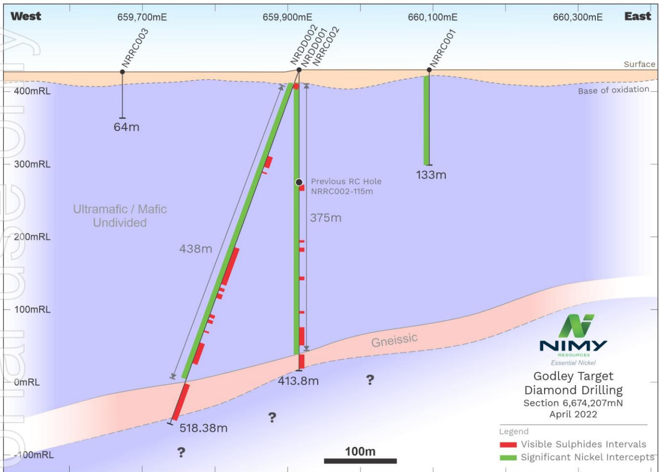
Figure 6 – Godley Target – Visible sulphide intervals and significant Nickel intercepts
