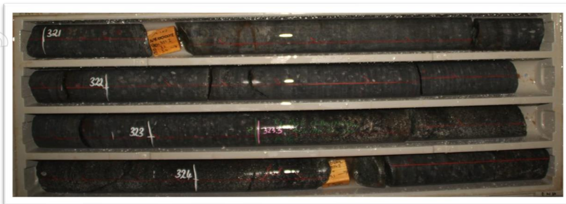
Figure 3 - Diamond Hole NRDD002 (Dry and wet) – Tray #91 - Disseminated sulphide (pentlandite 2%) from 323.3m to 327.4m
