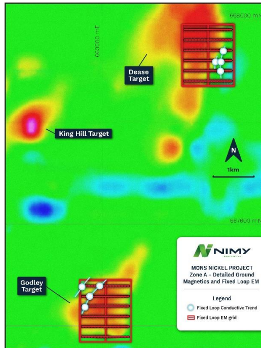
Figure 8 - Fixed Loop EM Conductive Trends located over the Godley and Dease Targets in Zone A
