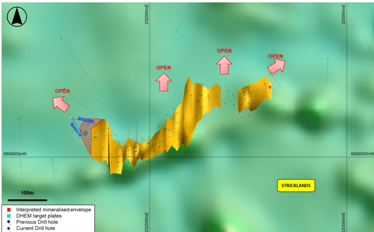
Figure 2 - plan view map (against magnetic data) with schematic of the mineralised envelope at Stricklands. The location of MAD209 and MAD210 is shown and the interpreted extension of the mineralised envelope to the north-west is highlighted.
