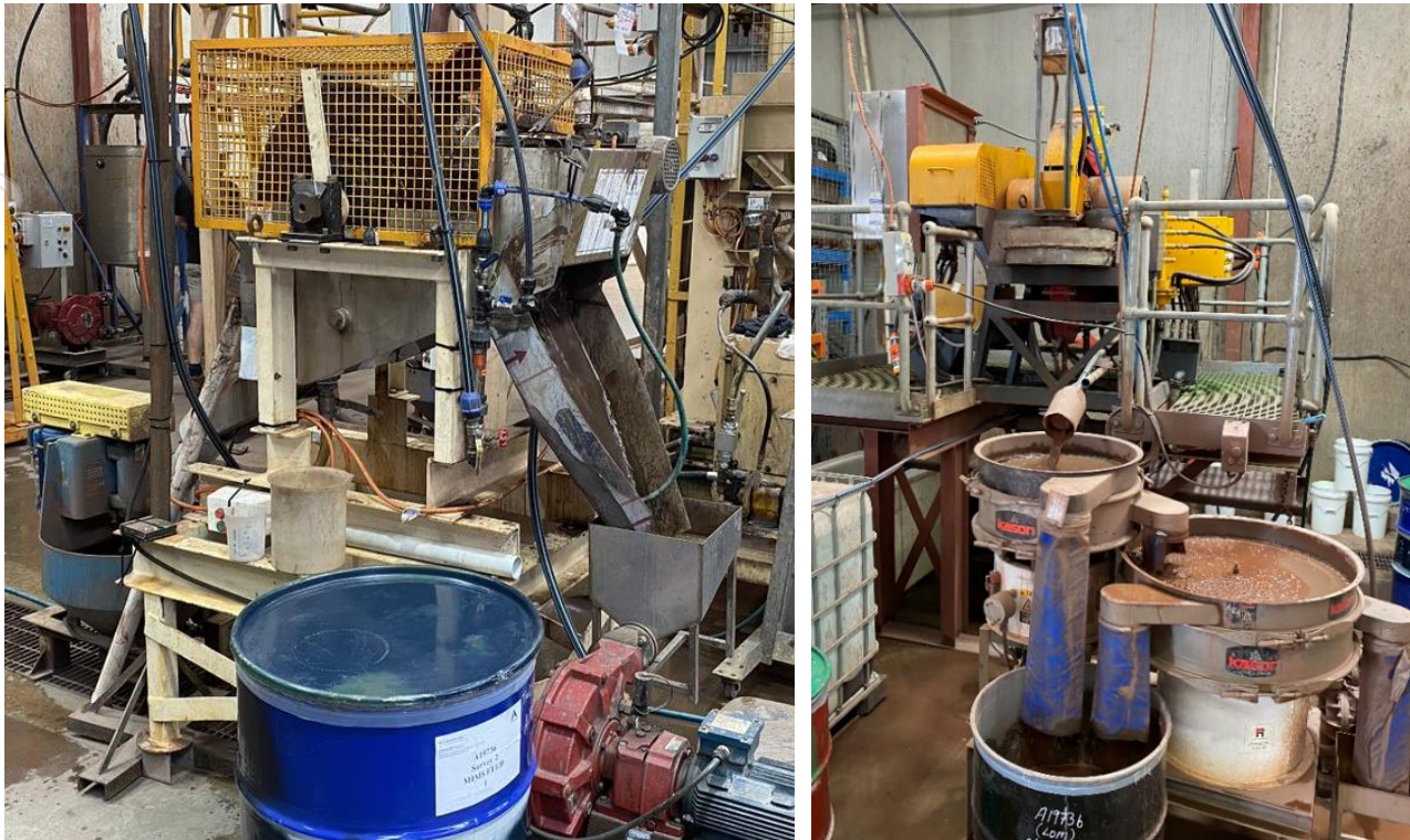
Figure 12 MIMS unit (left) and WHIMS unit (right)
