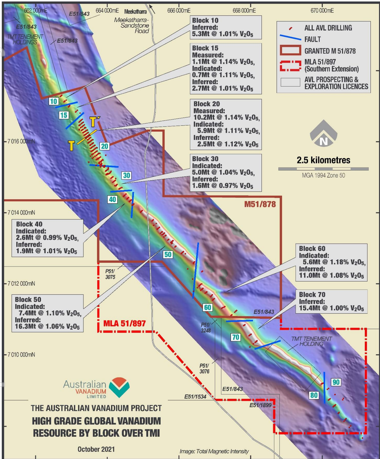
Figure 4 The Australian Vanadium Project Drilling, Fault Blocks and Section Locations on Total Magnetism Imagery
