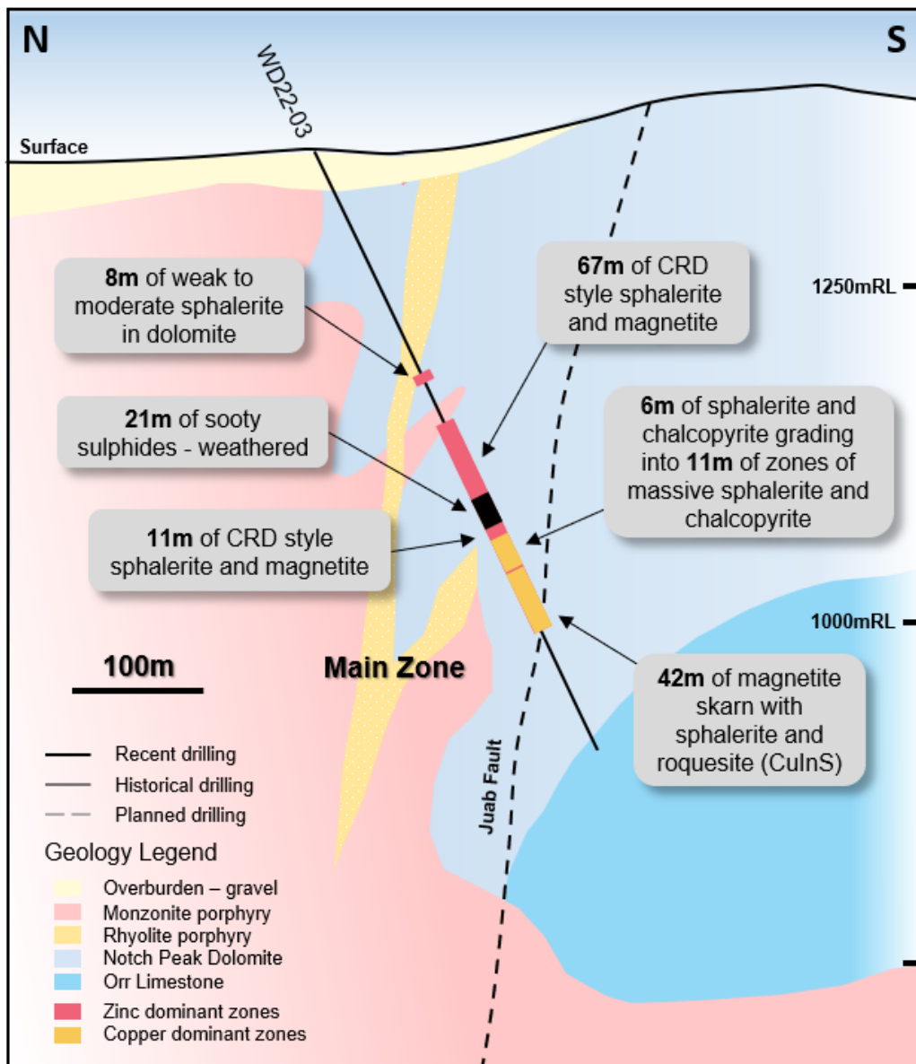
Figure 2: Schematic geological section at 289040E showing main geological units and drilling. The zinc and copper dominant mineralisation intersected in WD22-03 is shown.
