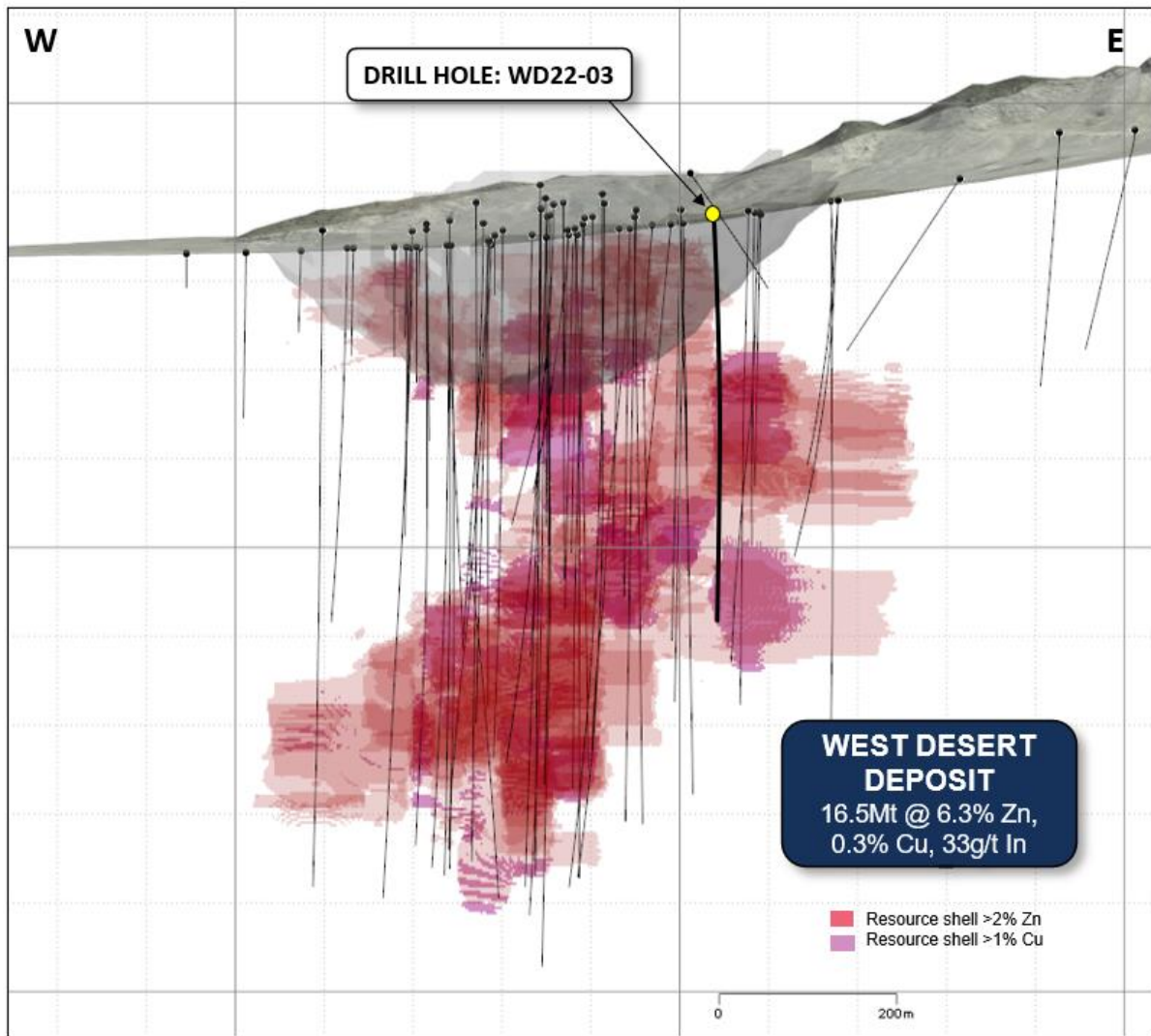
Figure 3: Long section view (looking north) of the West Desert Deposit (Red shading showing current >2% Zn ore blocks, purple shading showing current >1% Cu ore blocks), current open pit design and drilling. Drill hole WD22-03 is located close to the proposed open pit where underground development is expected to commence.
