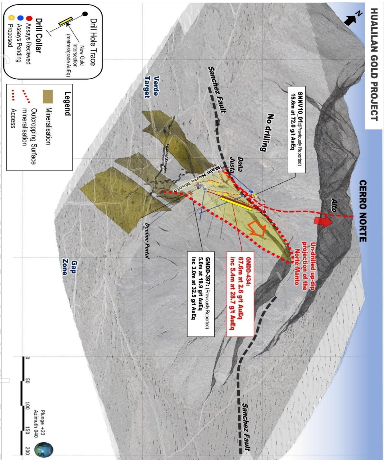
Figure 4 - 3D view of Cerro Norte showing the location of GNDD-397 and additional portable rig drilling
