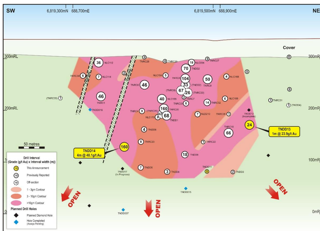
Figure 2: Hercules prospect long section showing significant drill hole gold interval pierce points and contours 3 .
