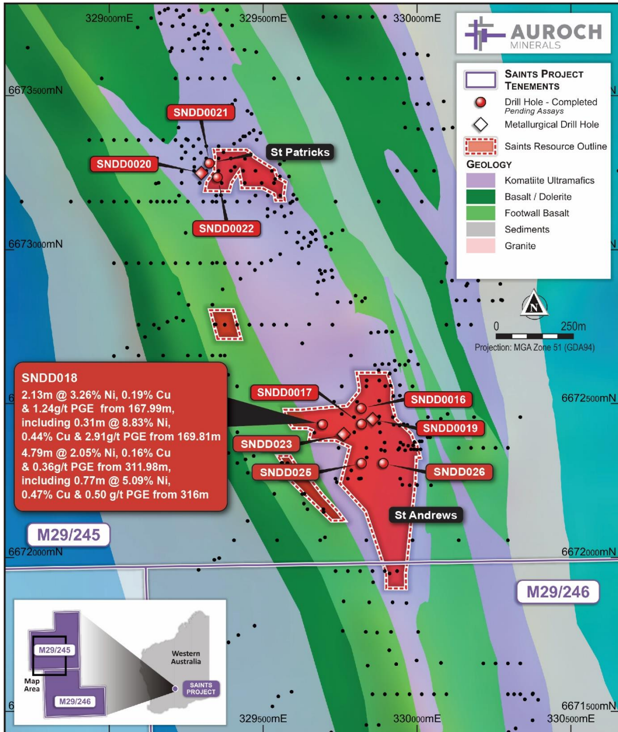
Figure 1 – Map of the Saints Nickel Project showing drill-hole SNDD018 and other completed drill-holes against interpreted geology and resource outline
