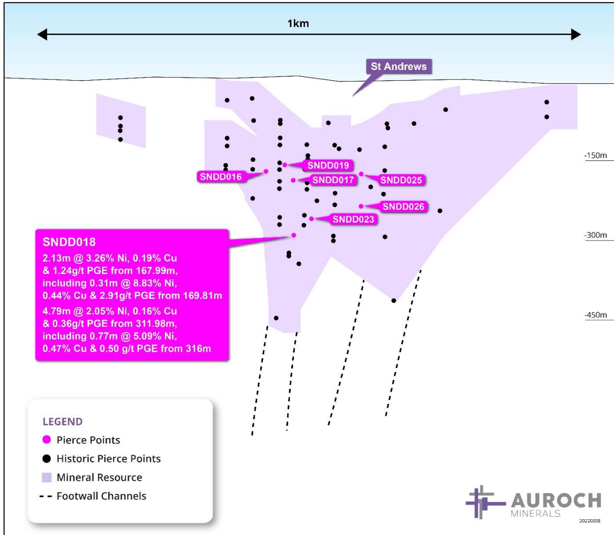
Figure 2 – Long-section of the current modelled resource at the Saint Andrews Prospect showing location of drill-hole SNDD018 and other pierce points from the current drill programme
