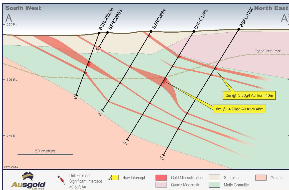
Figure 3 – Cross-section A-A' along Jackson – White Dam Lodes
