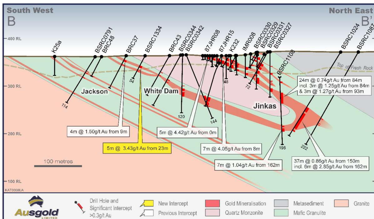
Figure 4 – Cross-section B-B' Jackson – White Dam Lodes
