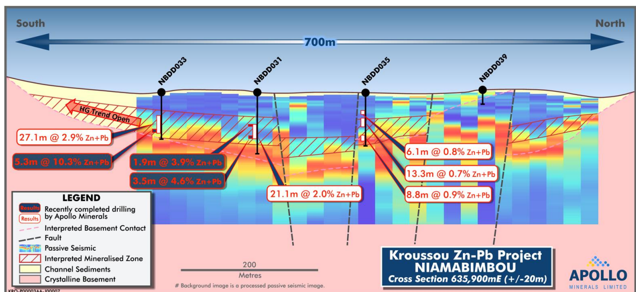
Figure 1: Section 635,900mE at Niamabimbou: Displaying maiden drilling with shallow high-grade mineralisation (overlaid on passive-seismic interpretation). Mineralisation is open to the south and east.
