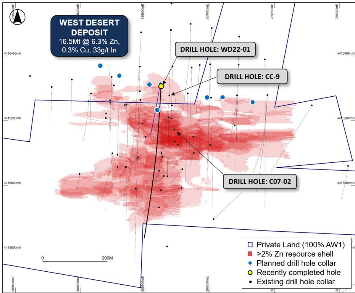
Figure 2: Plan view of the West Desert Deposit (Red shading showing current >2% Zn ore blocks) and drilling. Drill hole WD22-01 is located within a resource gap of ~ 90m, whilst also testing at depth and south of the deposit where there is very little drilling.
