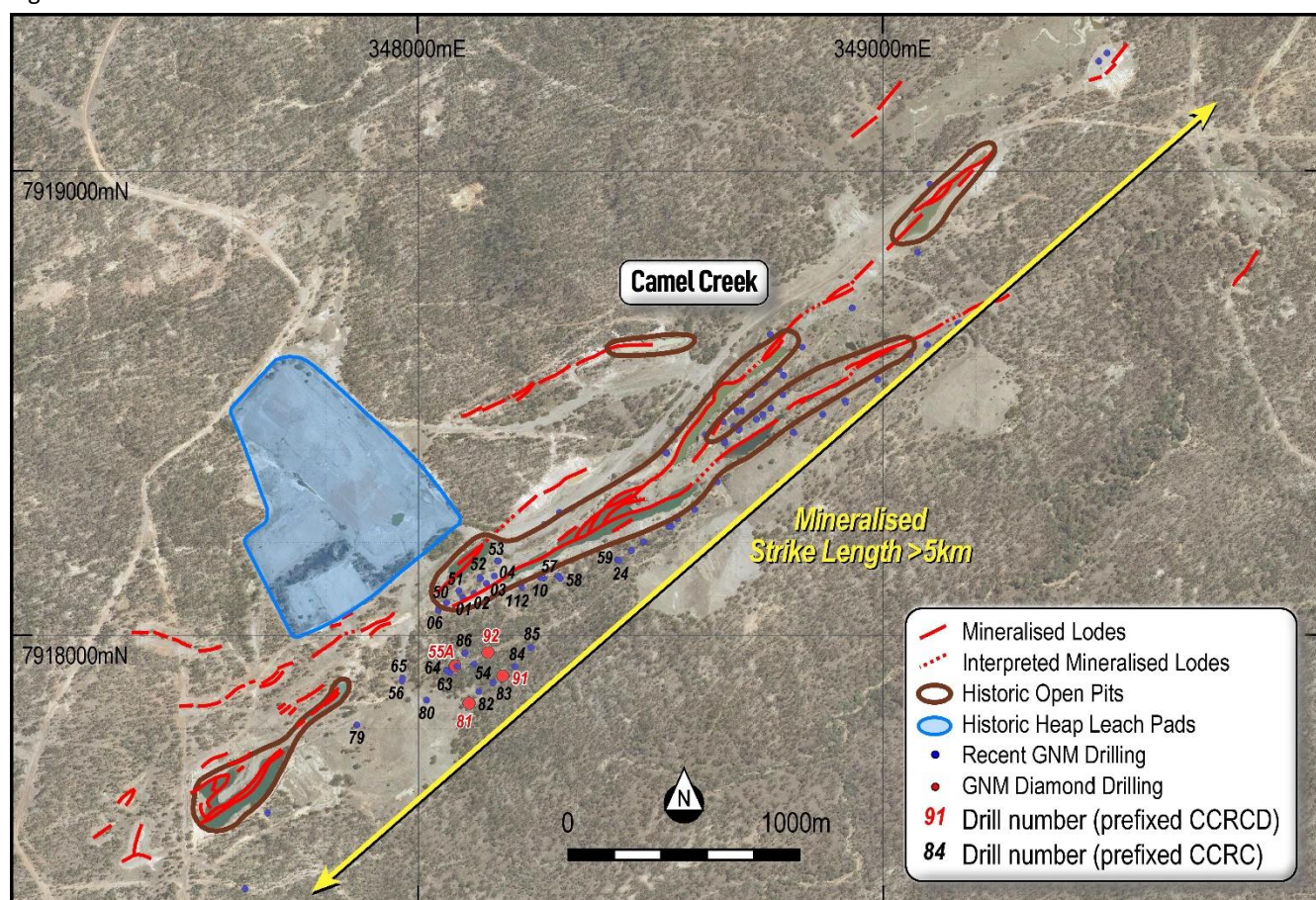
Figure 2 Camel Creek Plan
