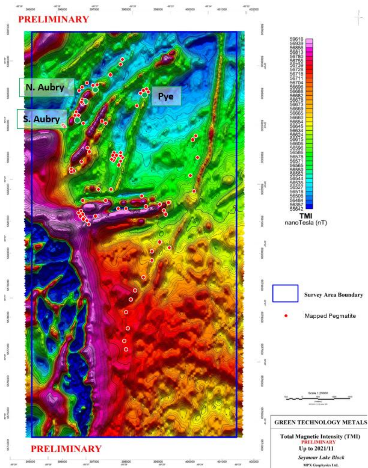
Figure 2: Plan image of Seymour Project overlain with Total Magnetic Intensity (TMI)
